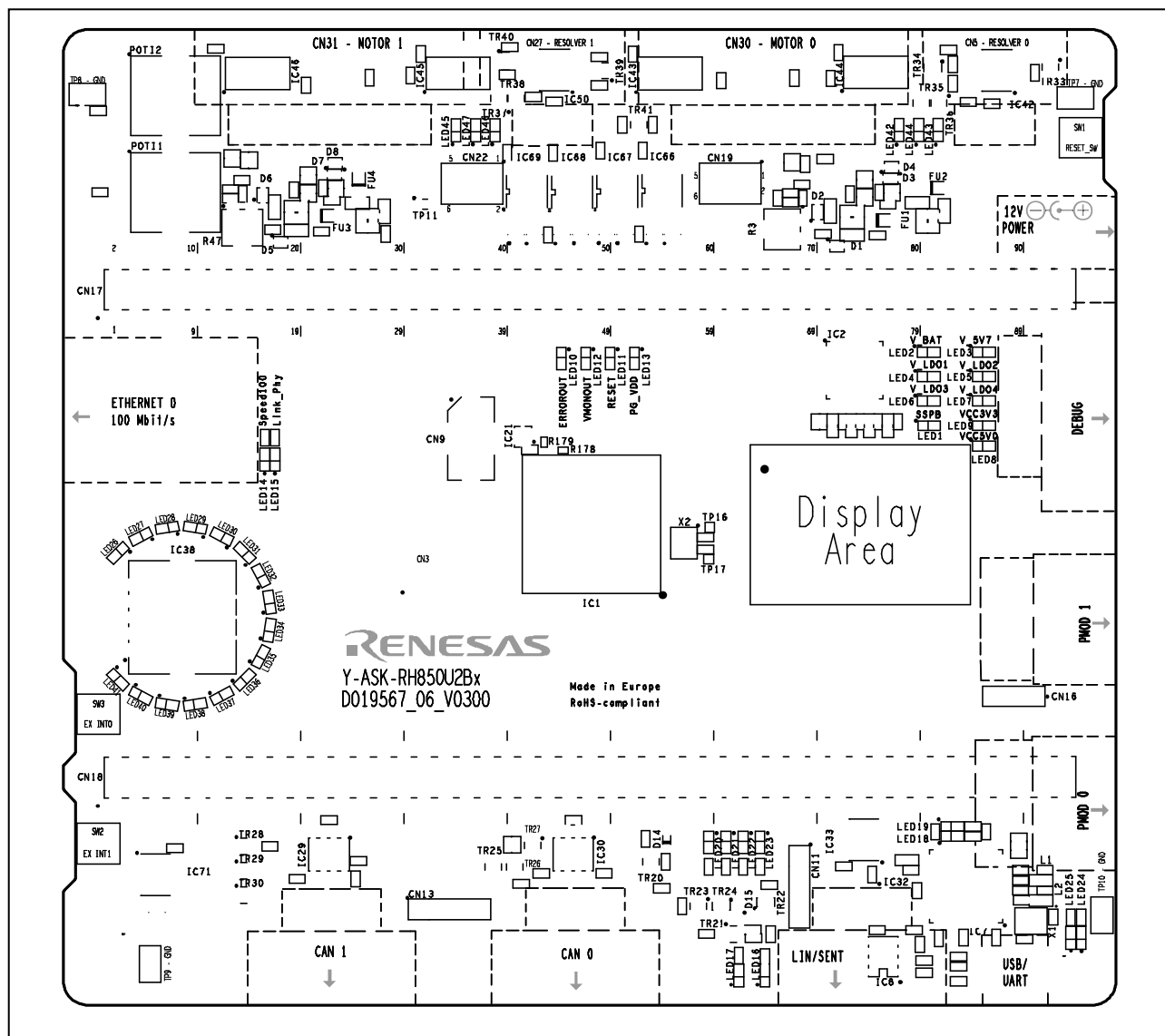
Figure 2.3 Placement of connectors and LEDs on top side of the starter for board version D019567_06_V0300
