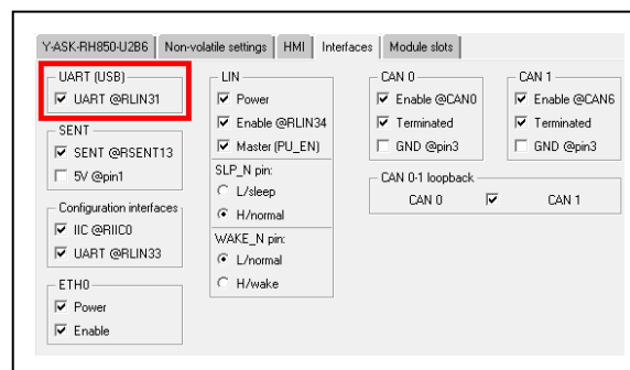
Figure 7.20 UART configuration
