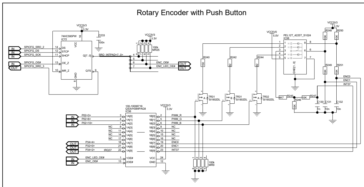
Figure 7.7 Rotary encoder
