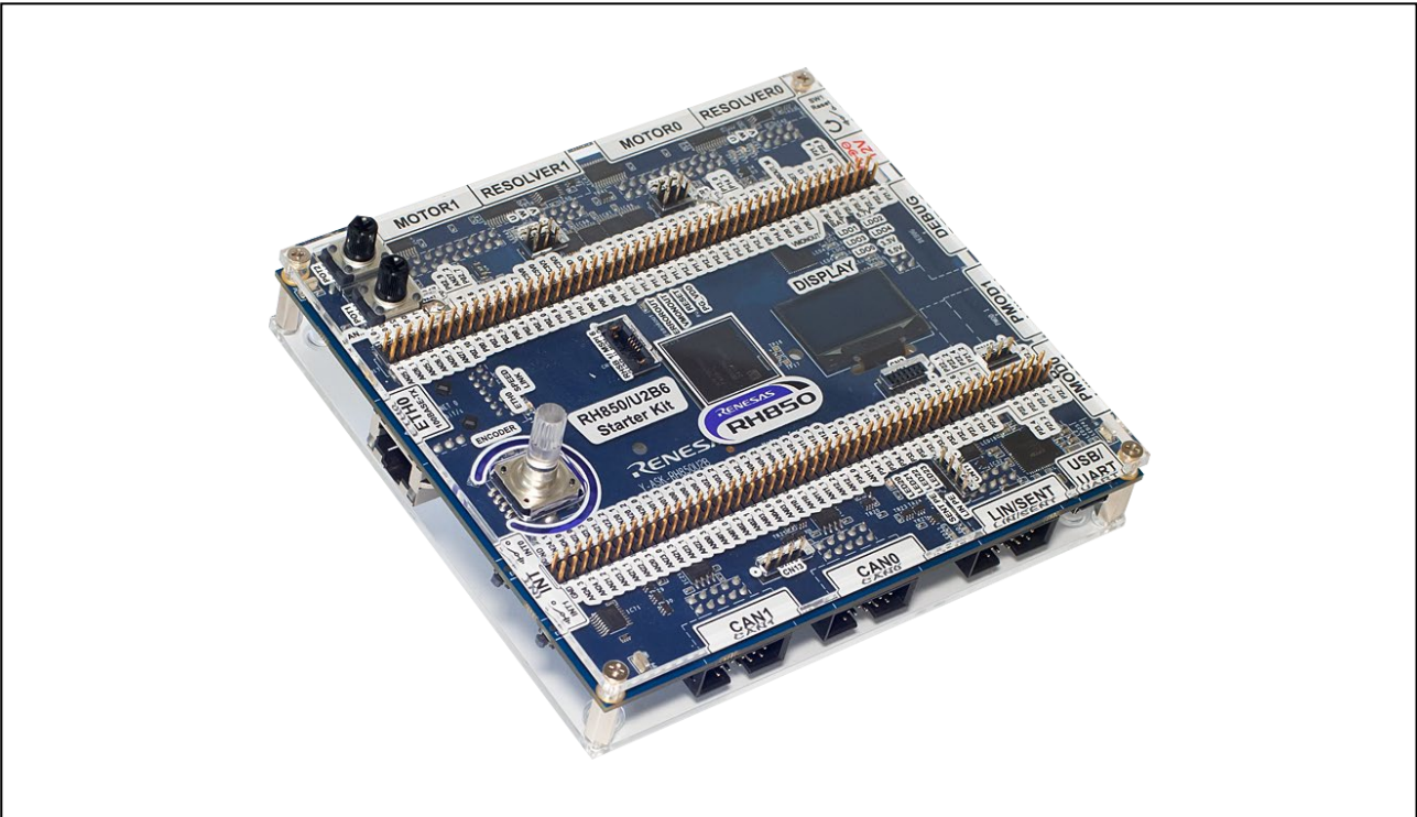
Figure 1.1 Starter kit
