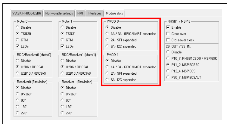
Figure 7.26 RHSB1 / MSPI6 enable
