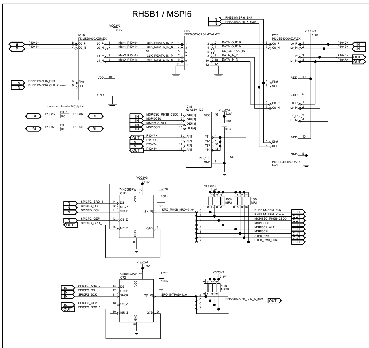
Figure 7.30 RHSB1 / MSPI6 interface
