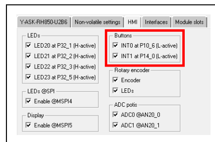
Figure 7.2 Interrupt input enable
