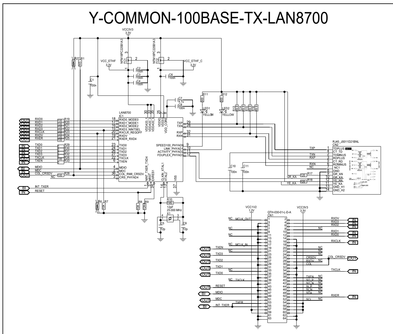
Figure 4.9 Circuit diagram of Renesas Ethernet board Y-COMMON-100BASE-TX-LAN8700
