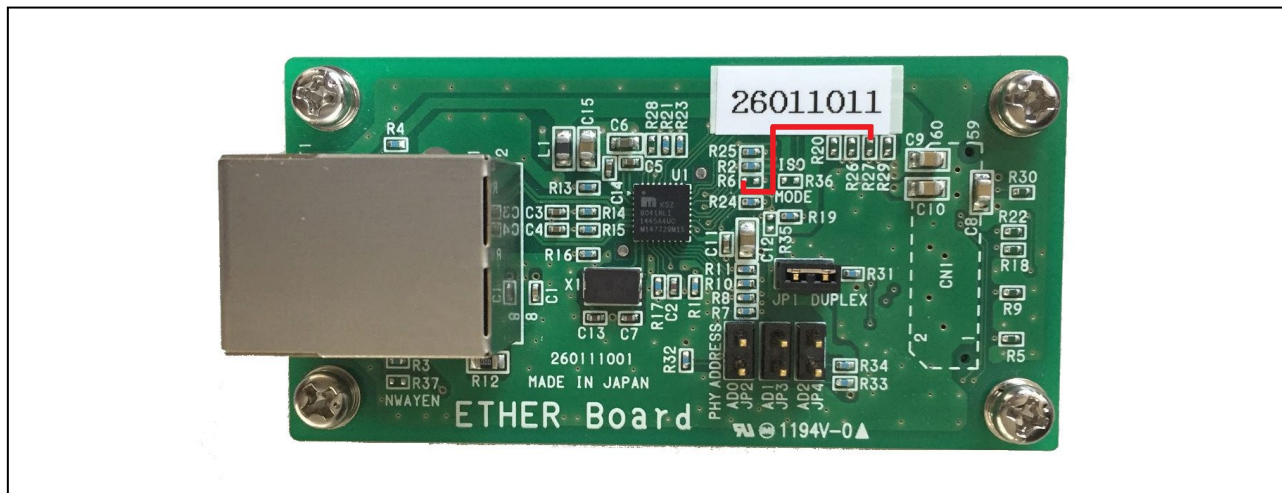
Figure 4.8 Modification of Shimafuji ETHER Board
