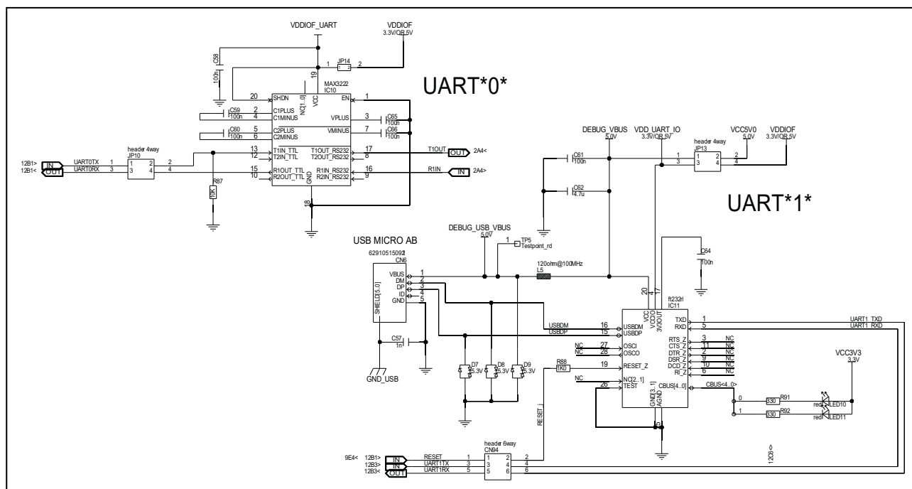
Figure 4.5 UART interface circuit diagram
