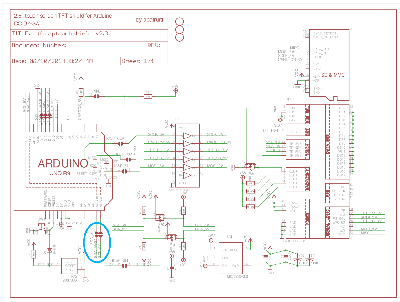
Figure 4.15 Touch display
