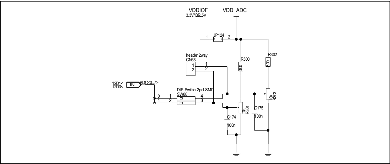
Figure 4.19 A/D measurements
