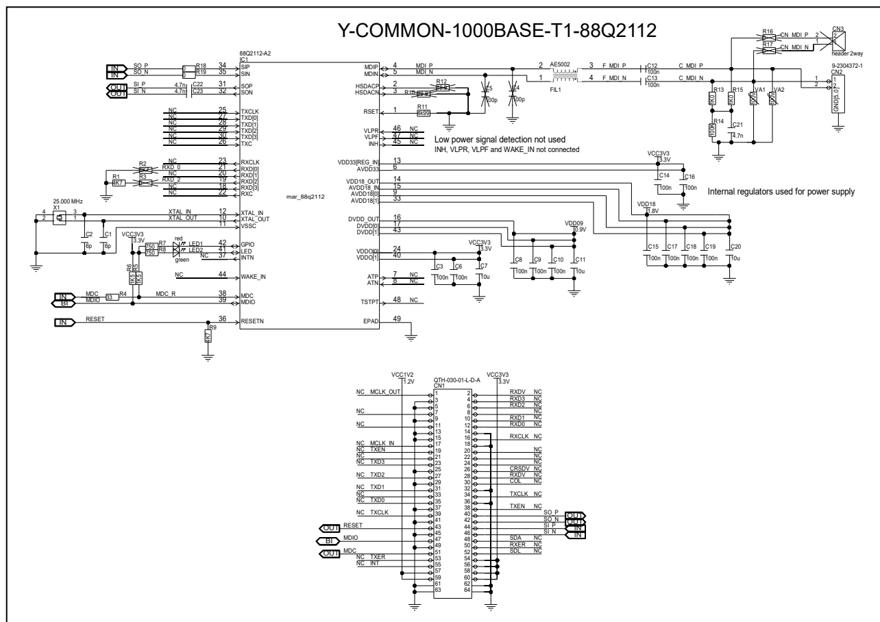
Figure 4.10 Circuit diagram of Renesas Ethernet board Y-COMMON-1000BASE-T1-88Q2112
