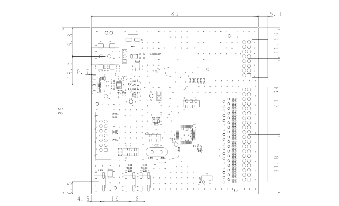
Figure 2-3. Board Dimensions
