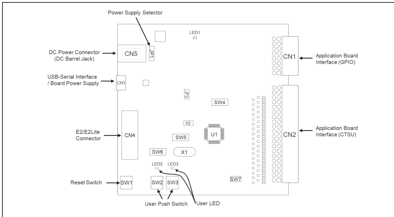
Figure 2-2. Parts Location
