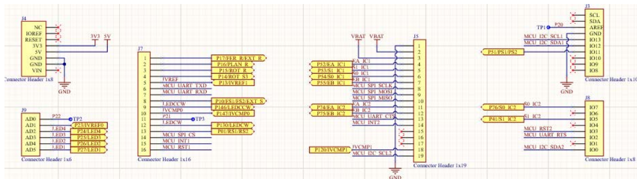
Figure 26. Header & Arduino connectors
