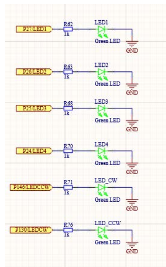
Figure 34. LEDs
