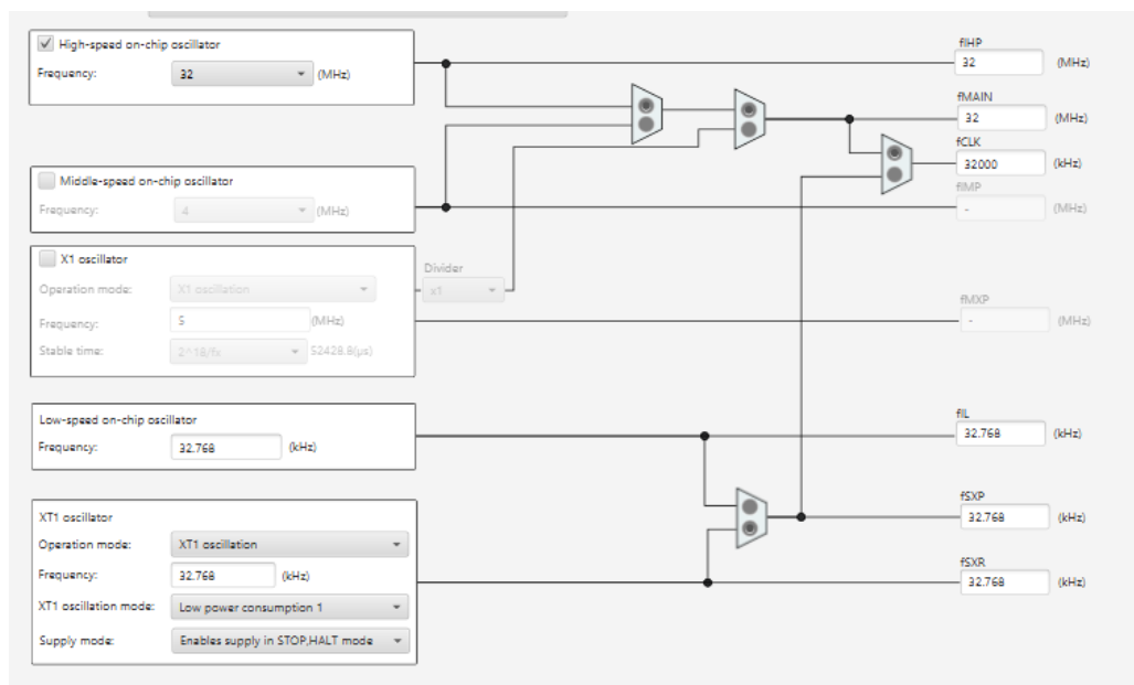
Figure 13. Clock tree
