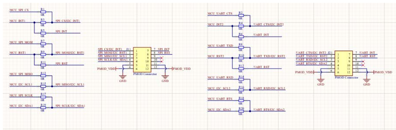
Figure 27. PMOD connectors
