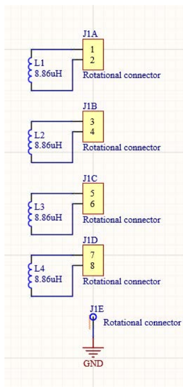
Figure 35. Rotation coils
