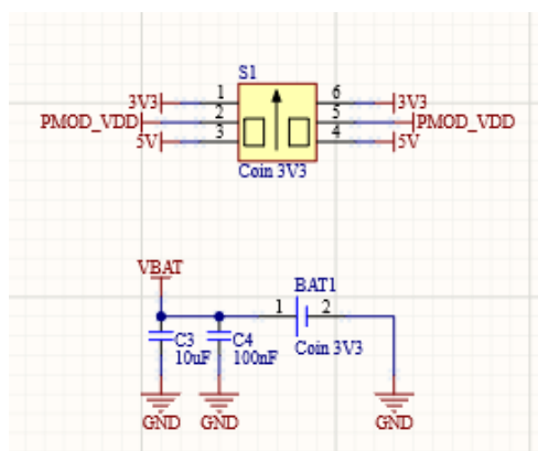
Figure 28. Supply options (+3V3 coin cell & PMOD supply switch)
