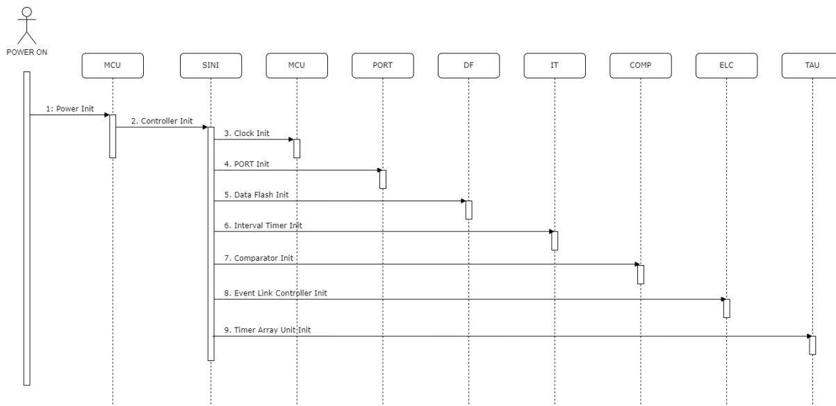
Figure 6. Activity diagram
