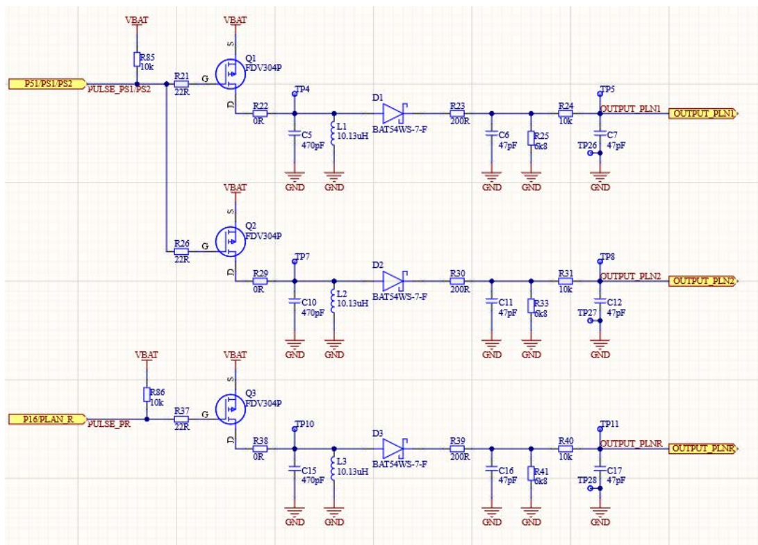
Figure 30. Planar group
