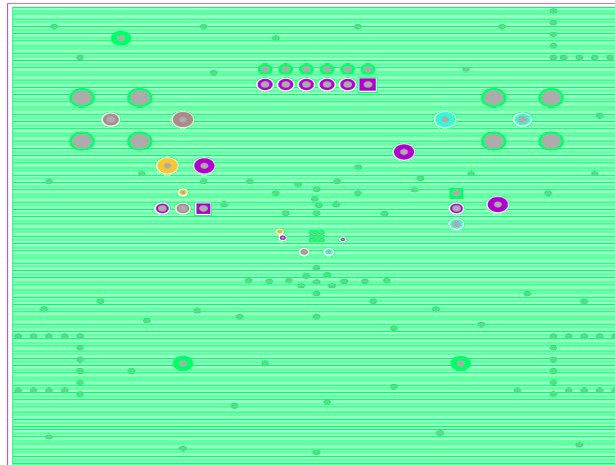
Figure 10. Bottom Layer
