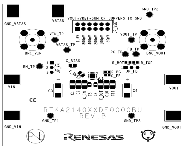
Figure 6. Assembly Layer
