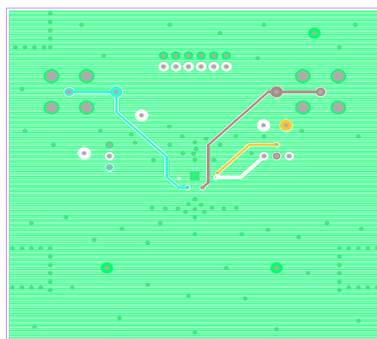
Figure 9. Third Layer
