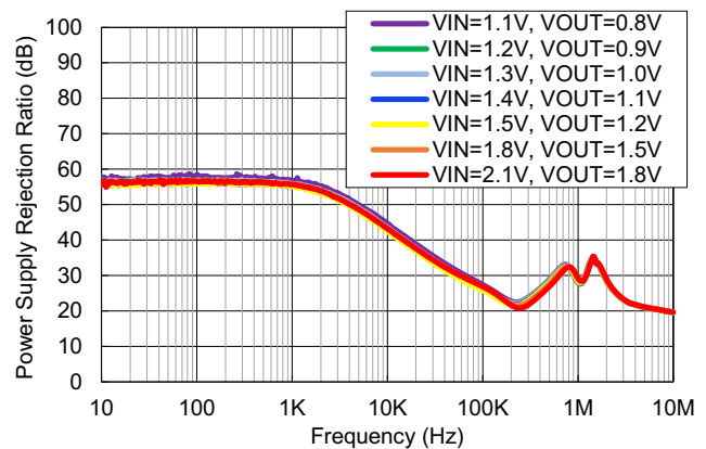
Figure 12. PSRR vs Frequency for Various V_{\text{OUT}} ( V_{\text{IN}} = V_{\text{OUT}} + 0.3\text{V} , V_{\text{BIAS}} = 5\text{V} , I_{\text{OUT}} = 3\text{A} , C_{\text{NR/SS}} = 1\mu\text{F} )
