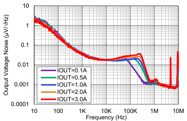
Figure 14. Output Voltage Noise for Various I_{\text{OUT}} ( V_{\text{IN}} = 1.4\text{V} , V_{\text{OUT}} = 0.8\text{V} , I_{\text{OUT}} = 3\text{A} , C_{\text{NR/SS}} = 0.1\mu\text{F} )
