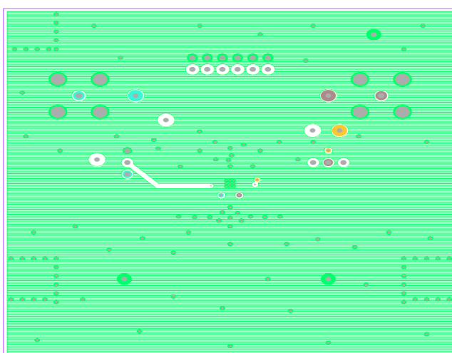
Figure 8. Second Layer
