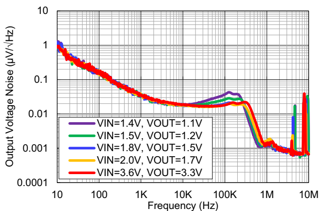
Figure 13. Output Voltage Noise for Various V_{\text{OUT}} ( V_{\text{IN}} = V_{\text{OUT}} + 0.3\text{V} , I_{\text{OUT}} = 3\text{A} , C_{\text{NR/SS}} = 1\mu\text{F} )
