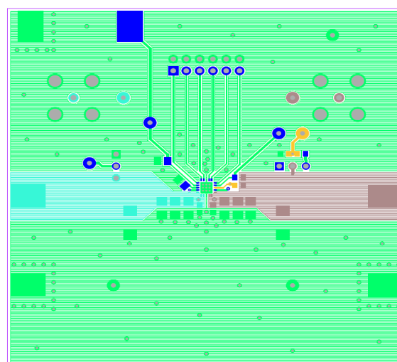
Figure 7. Top Layer
