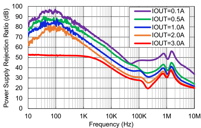
Figure 11. PSRR vs Frequency for Various I_{\text{OUT}} ( V_{\text{IN}} = 1.4\text{V} , V_{\text{OUT}} = 0.8\text{V} , C_{\text{NR/SS}} = 1\mu\text{F} )
