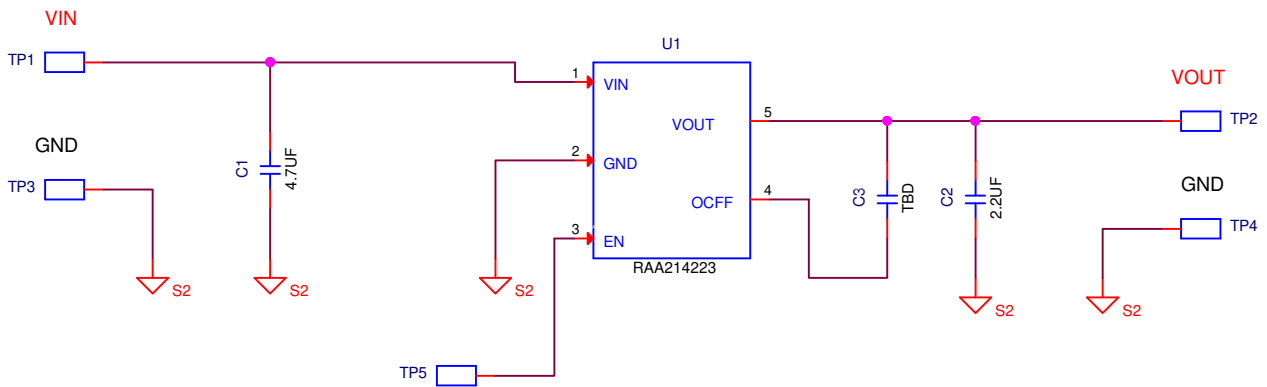
Figure 3. RTKA214223DR0000BU Schematic
