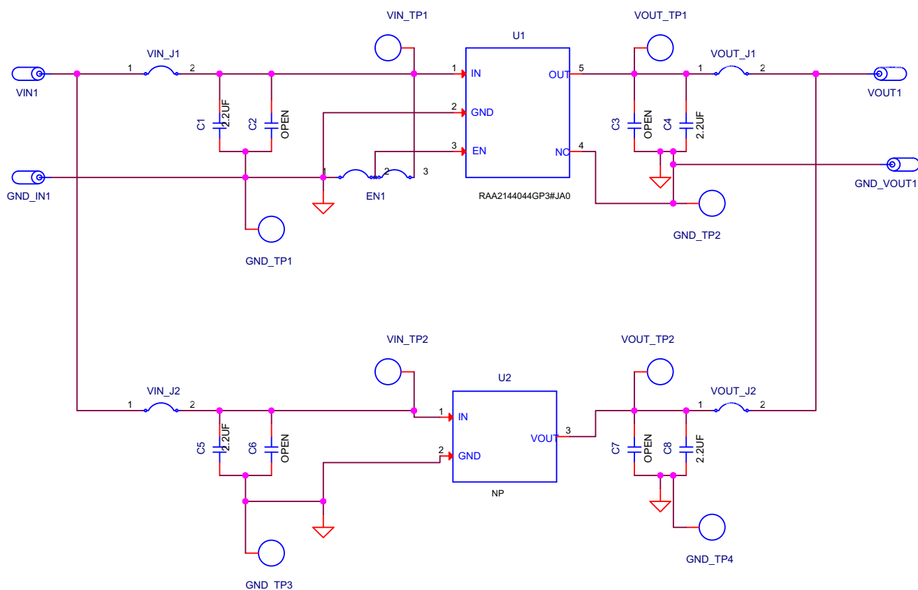
Figure 3. RTKA214404DE0000BU Schematic
