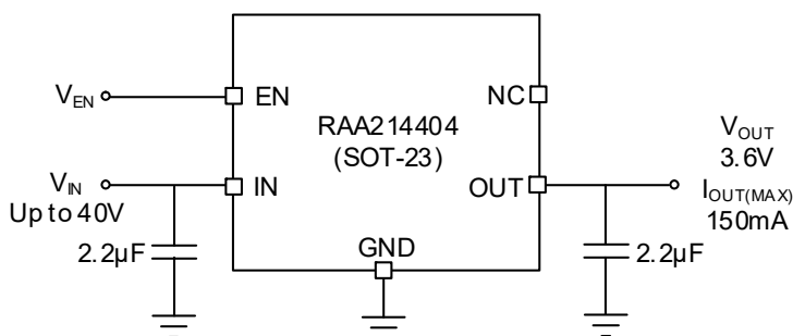
Figure 1. Block Diagram
