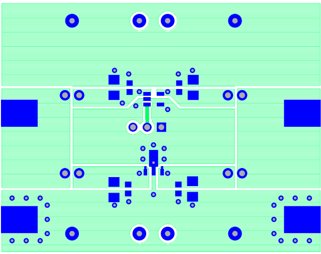
Figure 5. Top Layer
