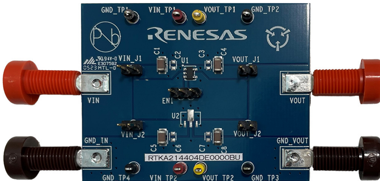
Figure 2. RTKA214404DE0000BU Board
