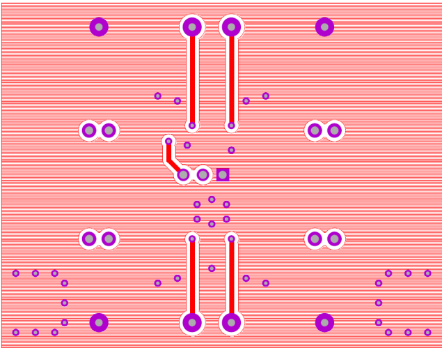
Figure 6. Bottom Layer
