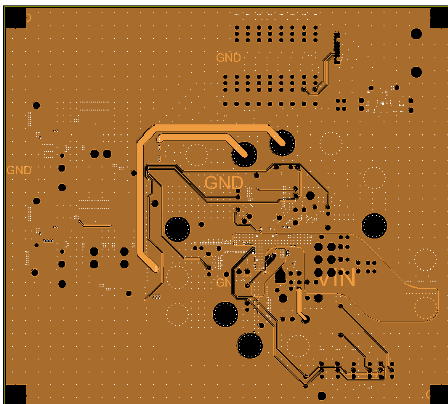
Figure 24. Layer 5 Copper
