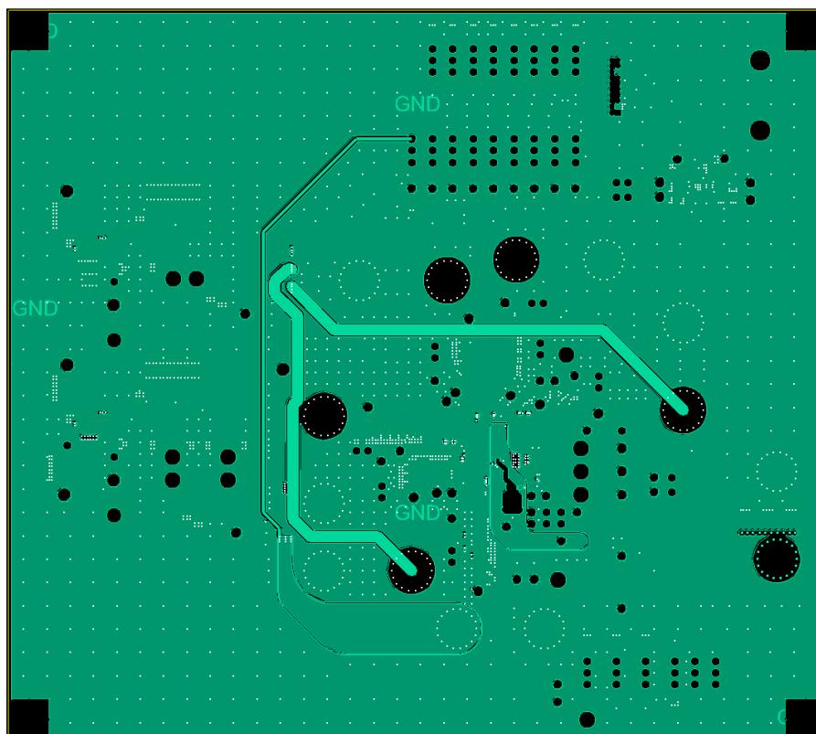
Figure 23. Layer 4 Copper
