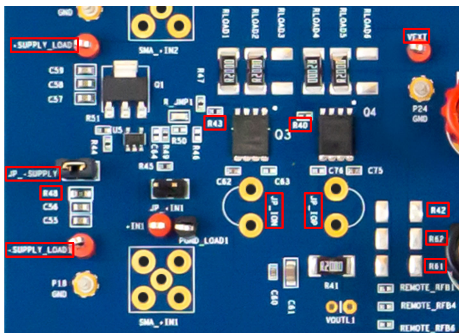
Figure 12. LOAD1 Configuration
