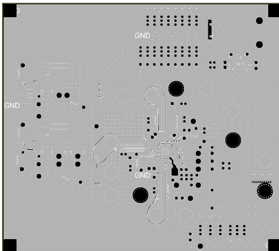
Figure 21. Layer 2 Copper
