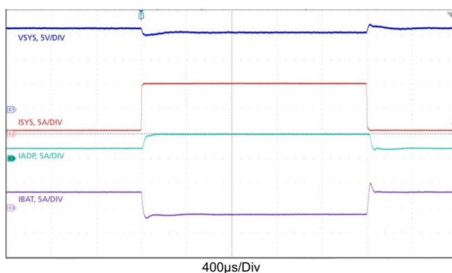
Figure 27. Buck Mode Transitions: Charge Current Loop to/from Adapter Current Loop. VADP = 28V, VBAT = 15.5V, MaxSystemVoltage = 16.768V, AdapterCurrentLimit = 5A, ChargeCurrent = 3A, SystemLoad: 0.5A \Leftrightarrow 10A
