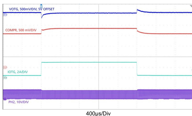
Figure 31. OTG Mode Transients. VBAT = 8V, VOTG = 5V, OTG Current = 4A, SystemLoad: 0.5 <=> 3A
