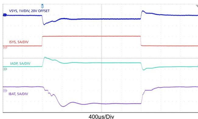
Figure 33. Bypass (HPBB) Mode, Reverse Turbo Boost Enabled. Charge Current Loop to/from Adapter Current Limit Loop Transitions, VADP = 20V, VBAT = 8V, MaxSystemVotlage = 8.384V, AdapterCurrentLimit = 3A, ChargeCurent = 2A, SystemLoad: 0.5 <=> 5A
