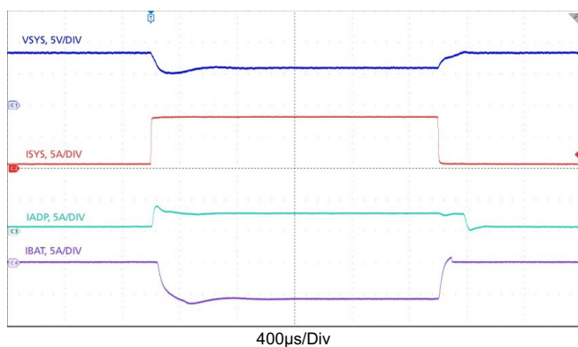
Figure 20. Boost Mode Transitions: Output Voltage Loop to/from Adapter Current Loop. VADP = 5V, VBAT = 7V, MaxSystemVoltage = 8.384V, AdapterCurrentLimit = 3A, ChargeCurrent = 0, SystemLoad: 0.5A \Leftrightarrow 8A
