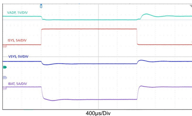
Figure 29. Boost Mode Transitions: Charge Current Loop to/from Input Voltage Loop. VADP = 5V, VBAT = 7.5V, MaxSystemVoltage = 8.384V, AdapterCurrentLimit Disabled, ChargeCurrent = 0.5A, SystemLoad: 0.5A \Leftrightarrow 8A, InputVoltageLimit = 4.48V
