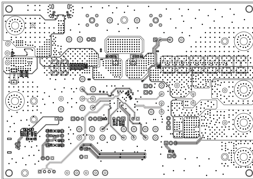
Figure 12. Bottom Layer
