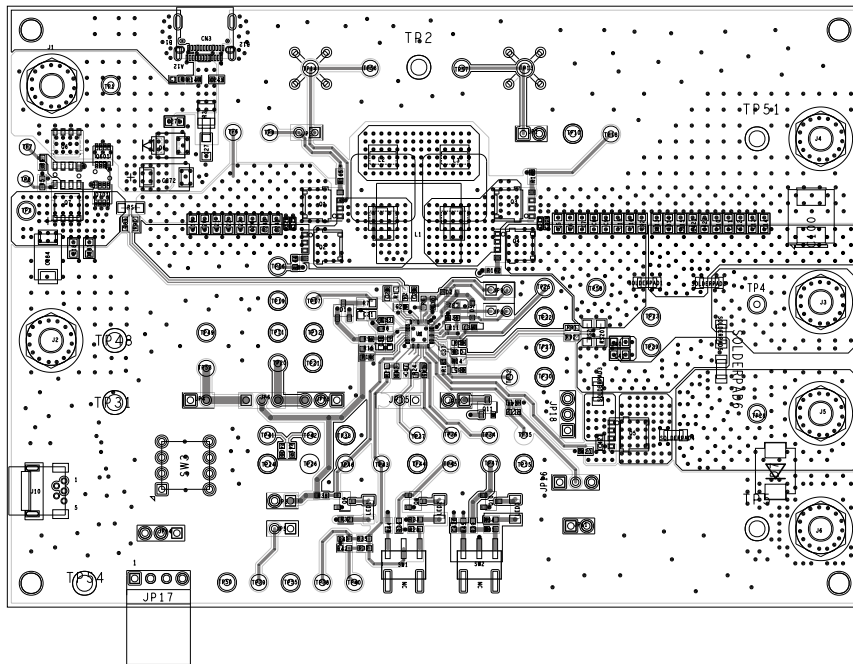
Figure 11. Top Layer
