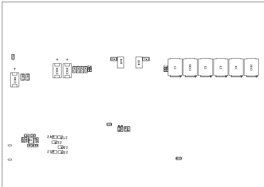
Figure 14. Bottom Silkscreen
