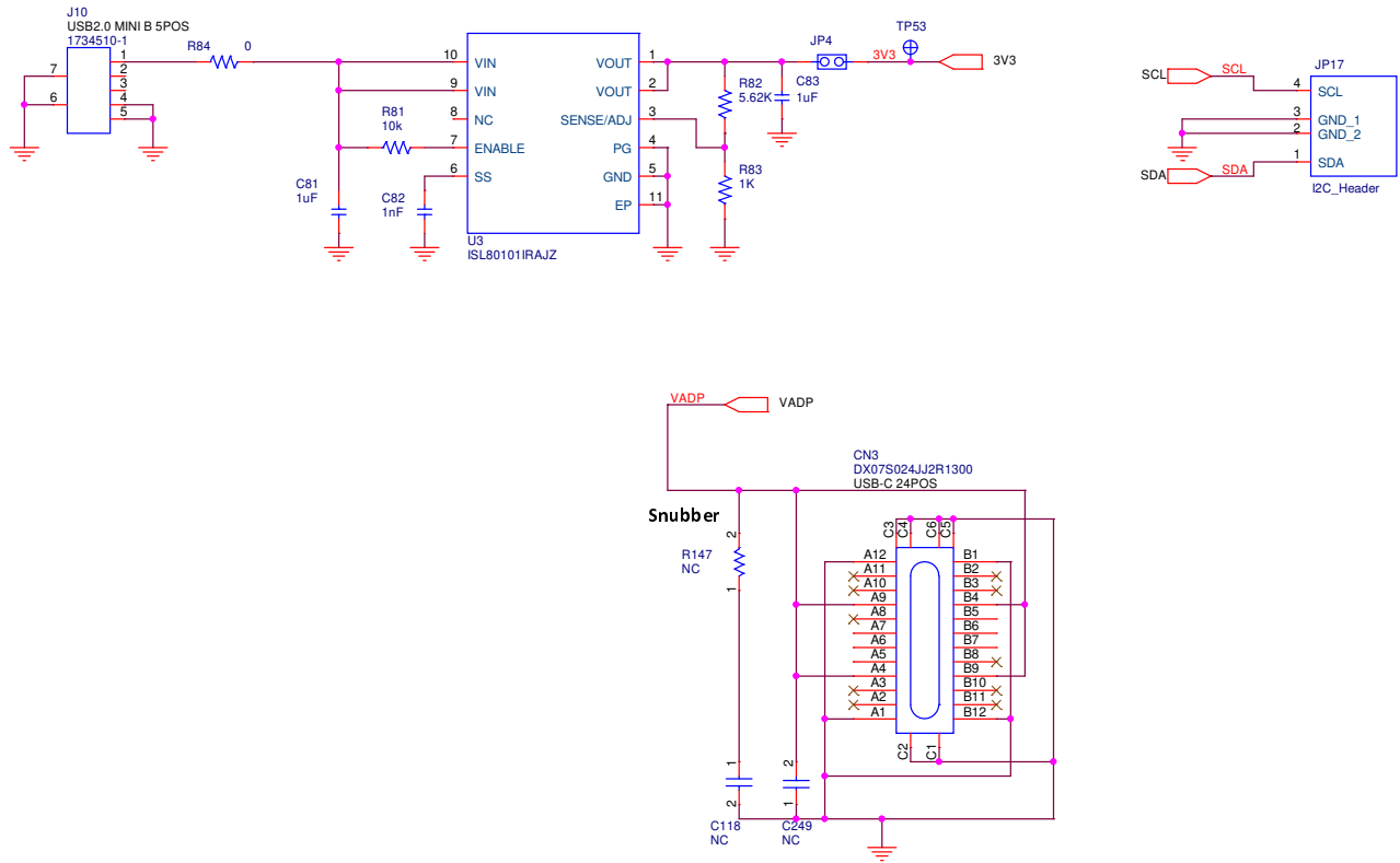
Figure 10. Schematic (2 of 2)
