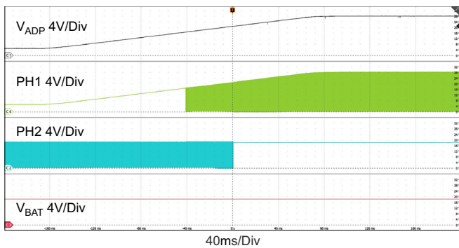
Figure 18. Adapter Voltage Ramp Up, Boost → Buck-Boost → Buck Operation Mode Transitions
