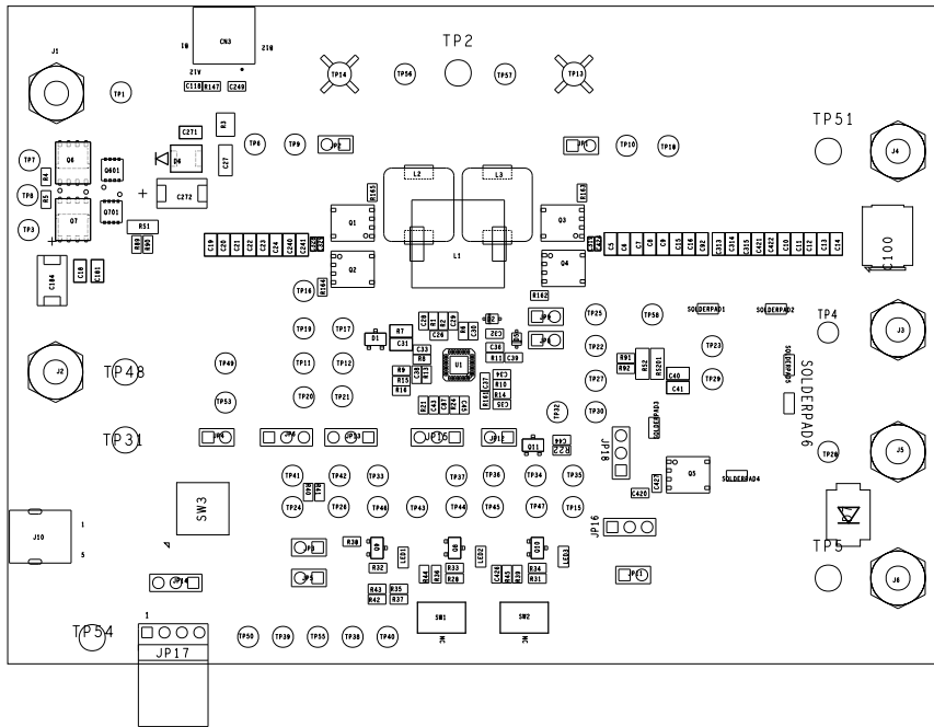
Figure 13. Top Silkscreen
