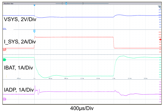
Figure 28. Buck-Boost Mode, Charging Current Loop to Adapter Current Loop Transition. V_{ADP} = 12V , MaxSystemVoltage = 12.576V , V_{BAT} = 11V , System Load 1A to 10A Step, AdapterCurrentLimit = 3A , ChargeCurrent = 1A
