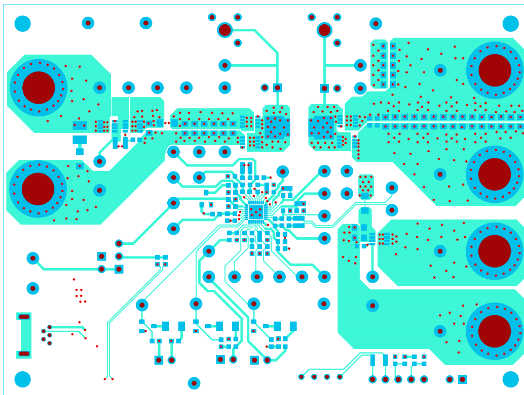
Figure 9. Top Layer
