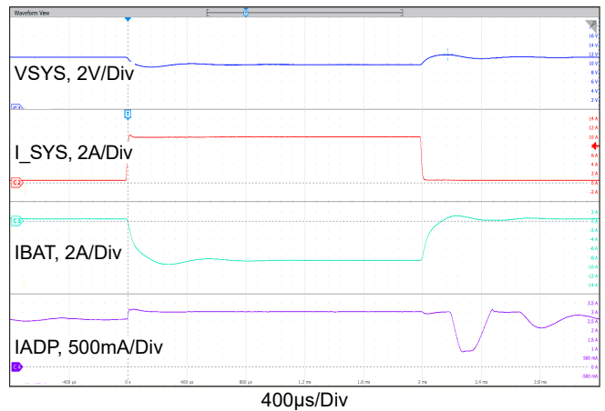
Figure 26. Boost Mode, Charging Current Loop to Adapter Current Loop Transition. V_{ADP} = 5V , MaxSystemVoltage = 12.576V , V_{BAT} = 11V , System Load 0.5A to 10A Step, AdapterCurrentLimit = 3A , ChargeCurrent = 0.5A
