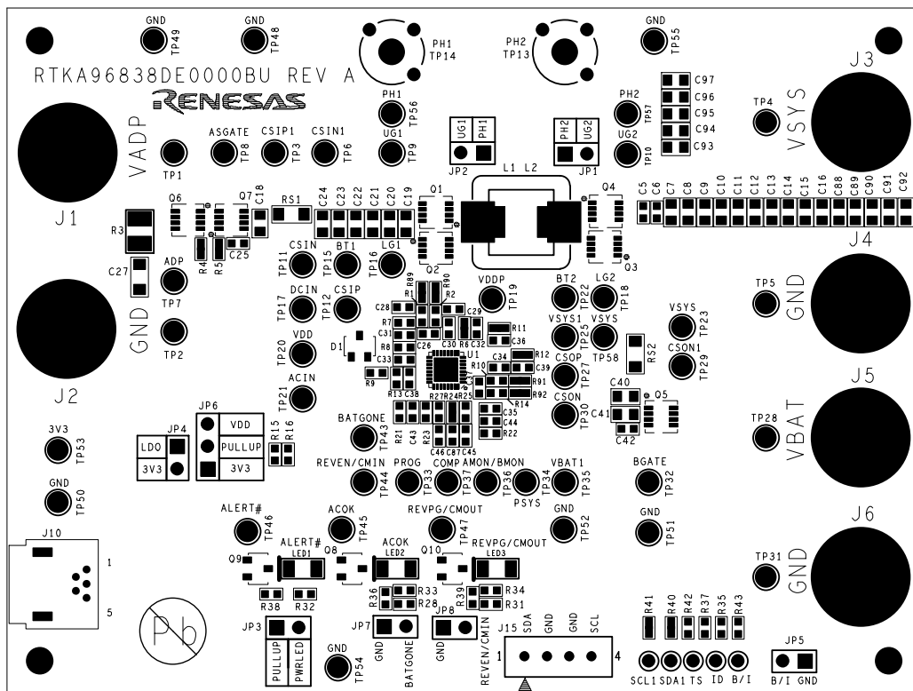
Figure 8. Top Silkscreen
