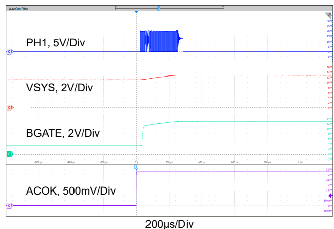
Figure 21. Adapter Insertion, V_{ADP} = 20V , V_{BAT} = 11V , ChargeCurrent = 0A (Figure 20 Zoomed In)
