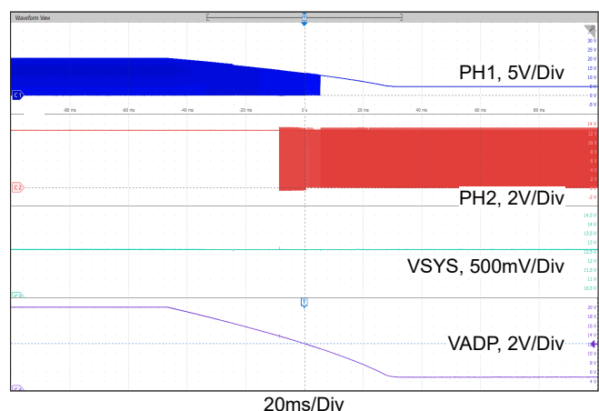
Figure 24. Adapter Voltage Ramps Down, Buck → Buck-Boost → Boost Operation Mode Transition
