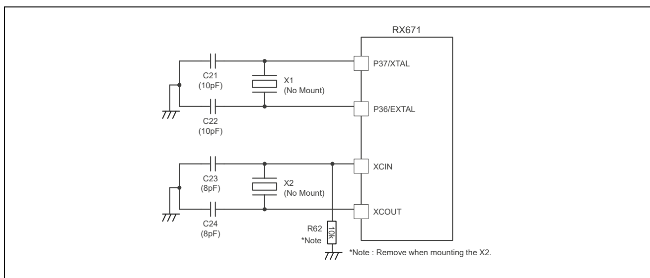
Figure 2-8. Clock Circuit
