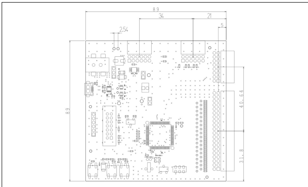
Figure 2-3. Board Dimensions
