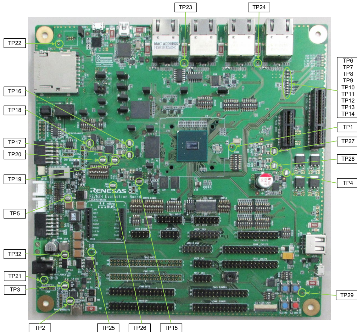
Figure 7-39 Arrangement of Test Pins
