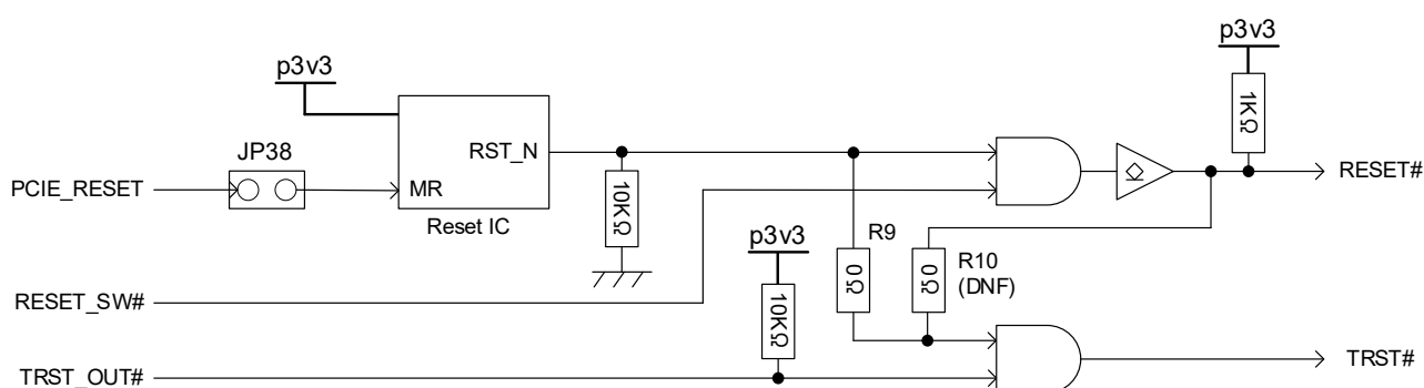
Figure 7-1 Configuration of Reset Circuit
