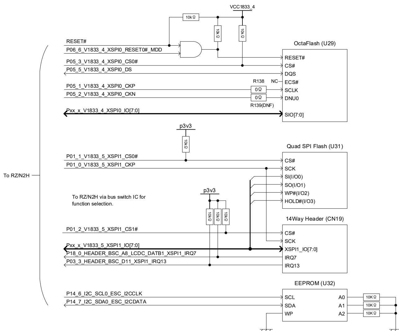
Figure 7-14 Configuration of SPI Memory Circuits
