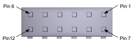
Figure 7-6 Pin Assignment for a Digilent Pmod™ Connector (Viewed from the Direction of Insertion)
