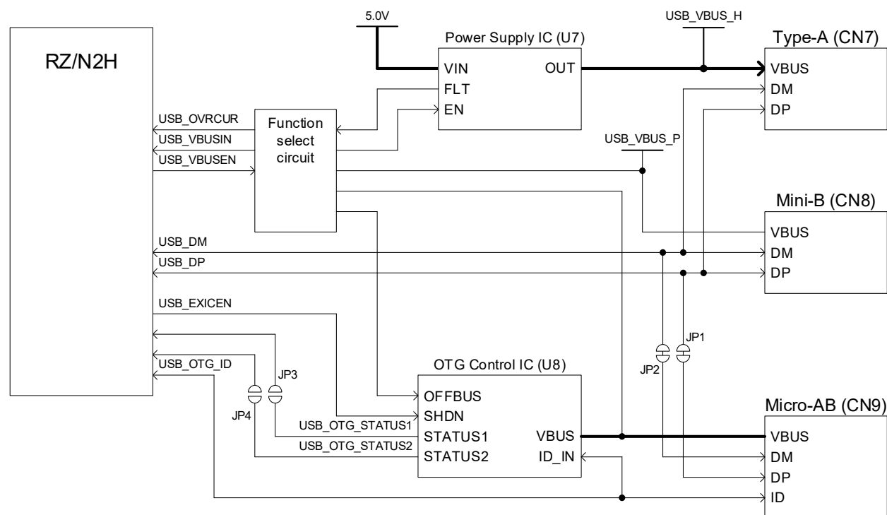
Figure 7-23 Configuration of USB Circuit
