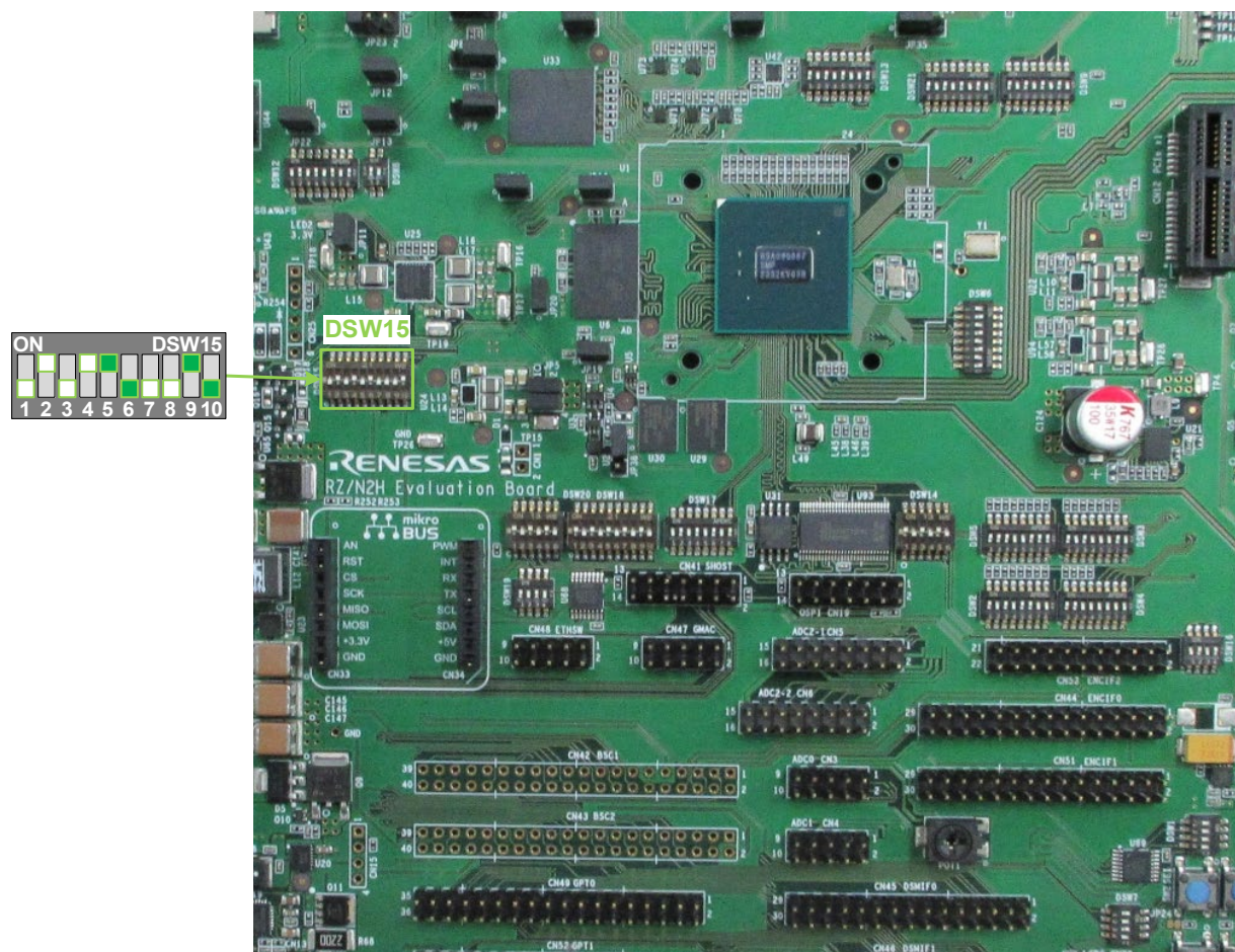
Figure 7-15 Switch Settings When Using EEPROM
