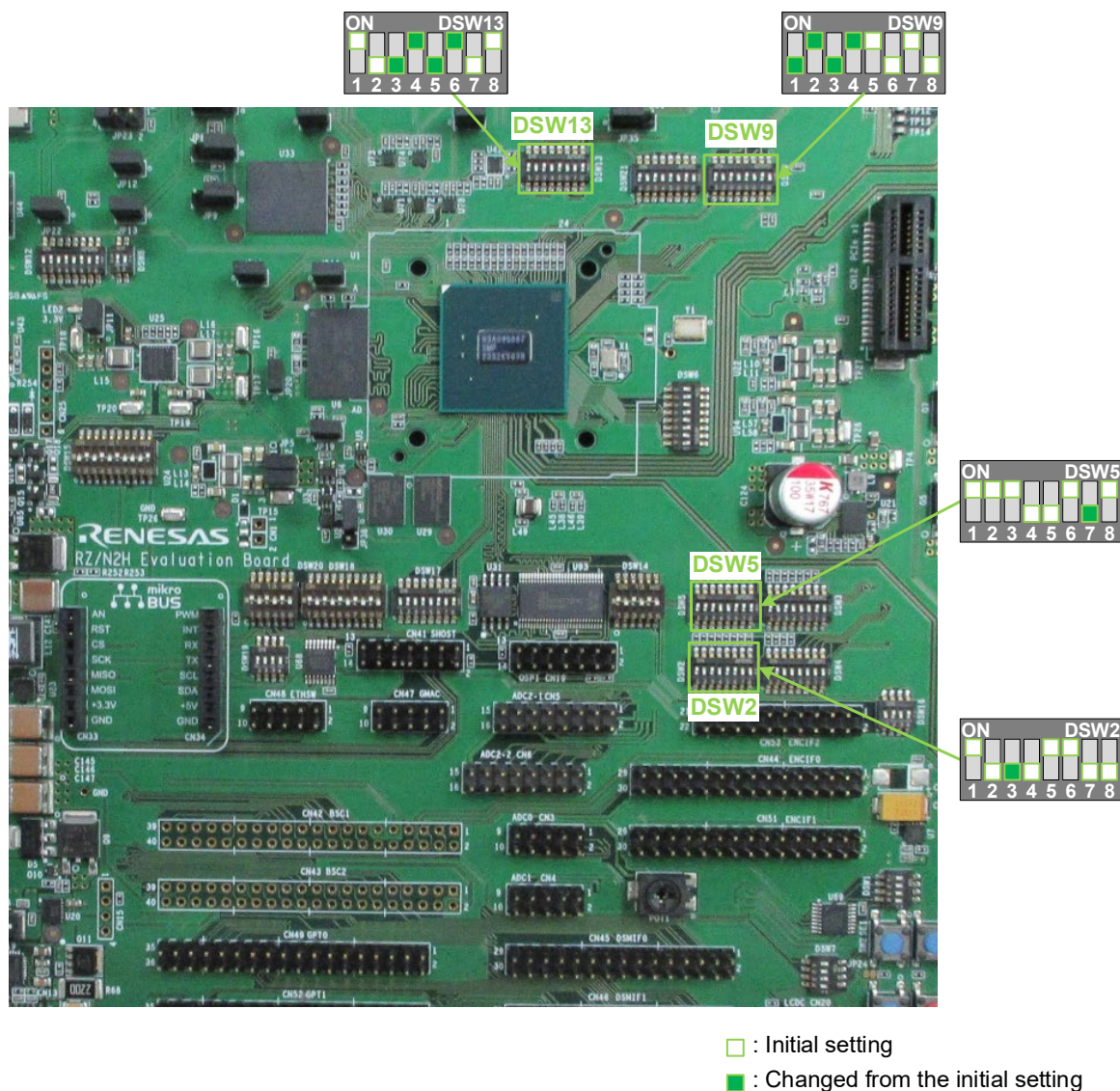
Figure 7-31 Switch Settings When Using the Serial Host Interface
