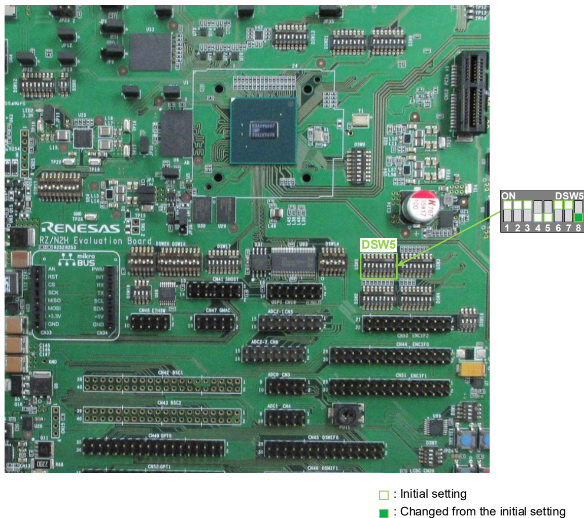
Figure 7-13 Switch Settings When Using USB-to-Serial Conversion Circuit
