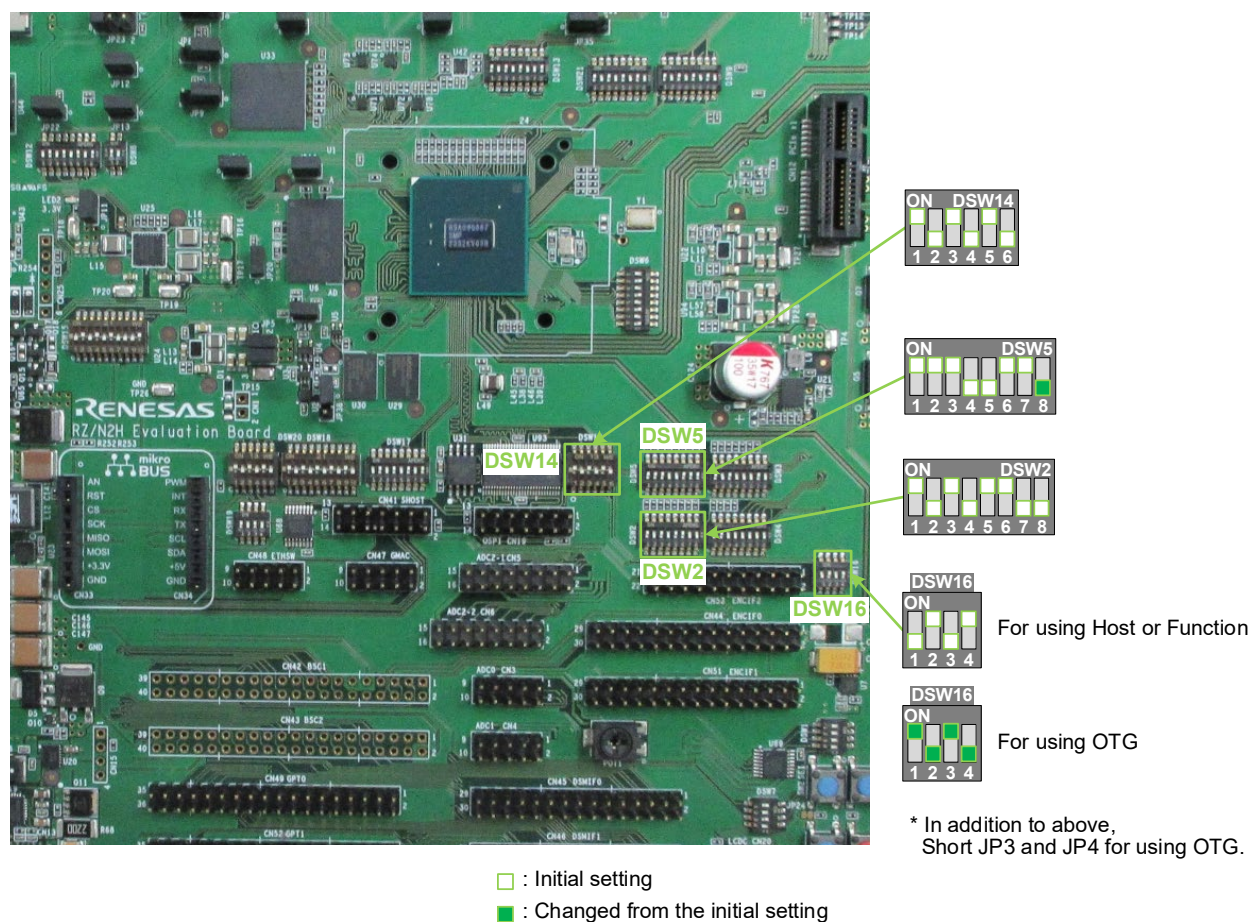
Figure 7-24 Switch Settings When Using USB Circuit (Port 00)
