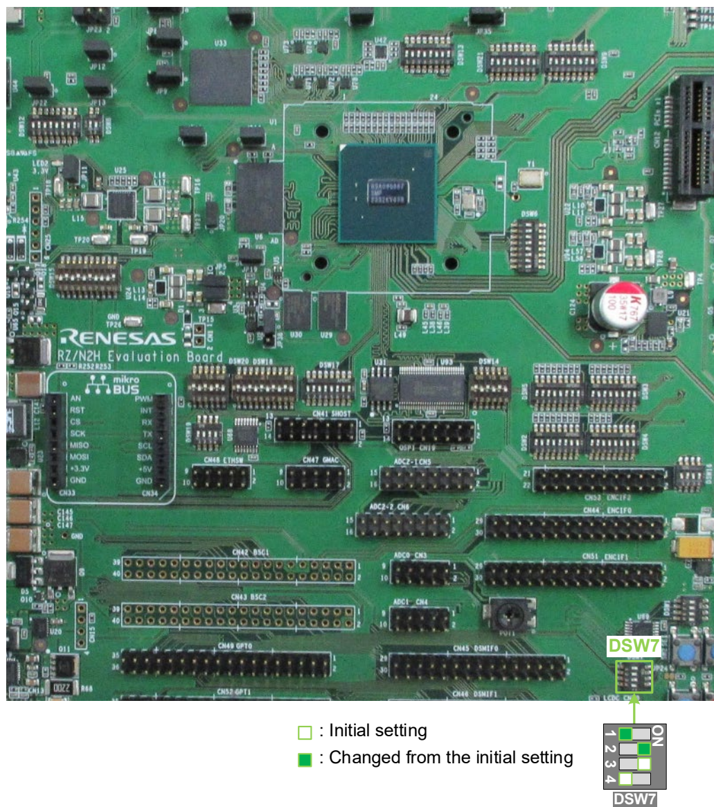
Figure 7-16 Switch Settings When Using SPI Expansion Connector (CN19)
