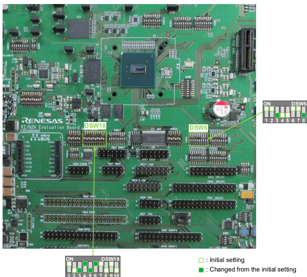
Figure 7-11 Switch Settings When Using mikroBUS™
