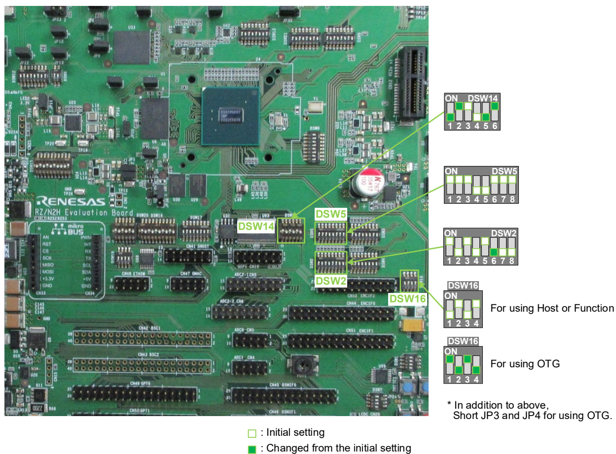
Figure 7-25 Switch Settings When Using USB Circuit (Port 02)
