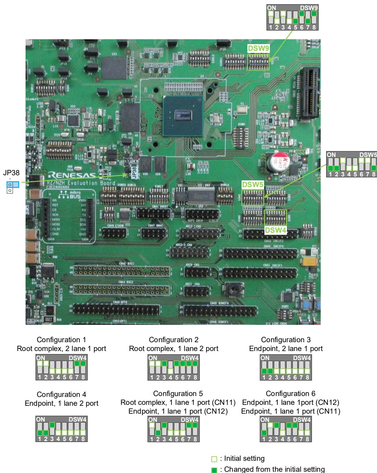
Figure 7-28 Switch Settings When Using PCIe
