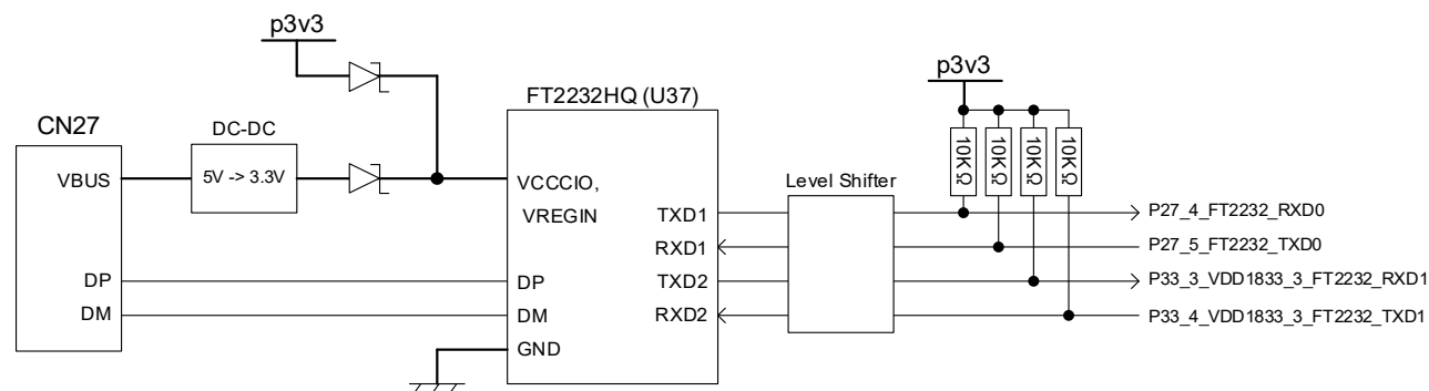
Figure 7-12 Configuration of USB-to-Serial Conversion Circuit
