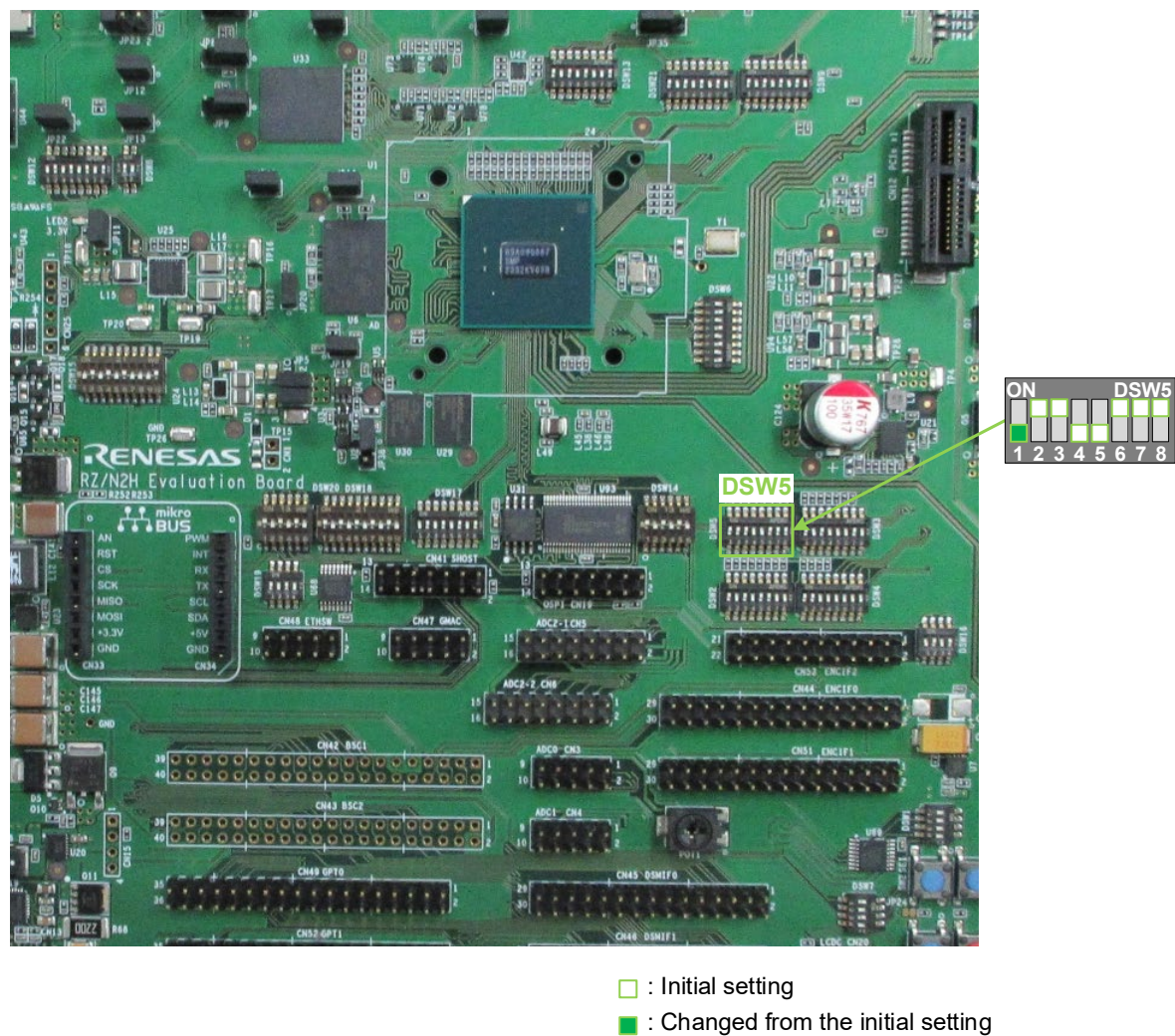
Figure 7-19 Switch Settings When Using the SD Card Slot (CN21)
