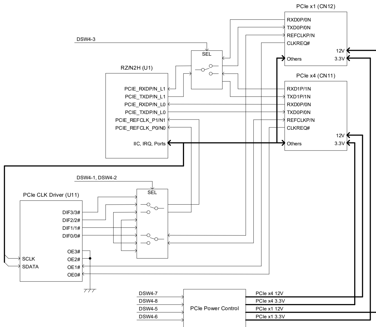
Figure 7-27 Configuration of PCIe Circuit
