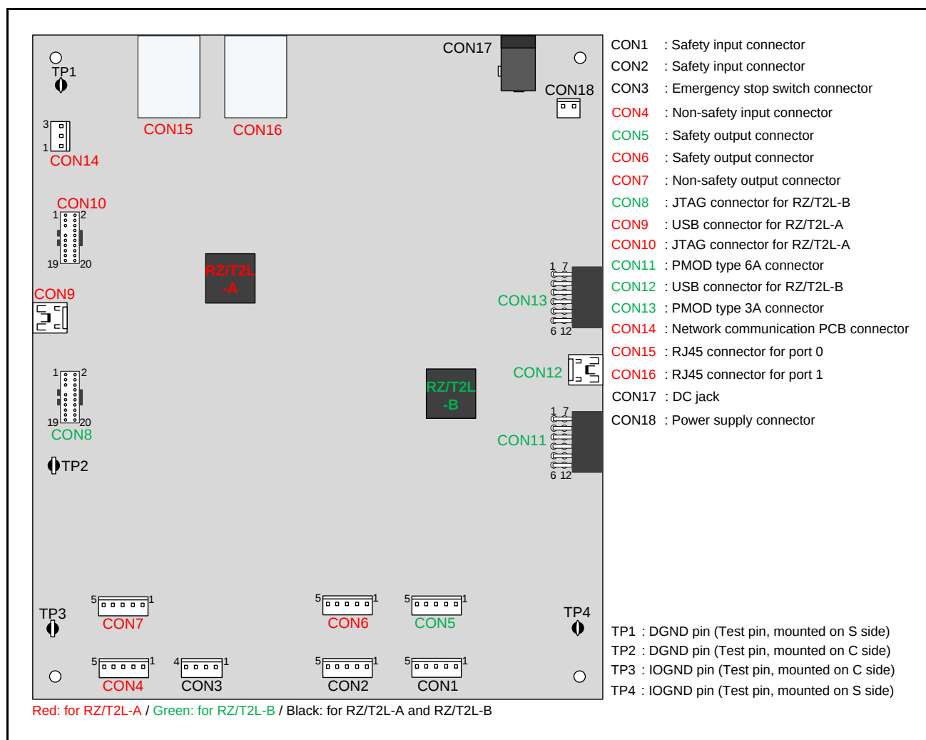
Figure 4.1.1 Functional Safety Reference Board - Connectors and Test Pins (C Side Up)
