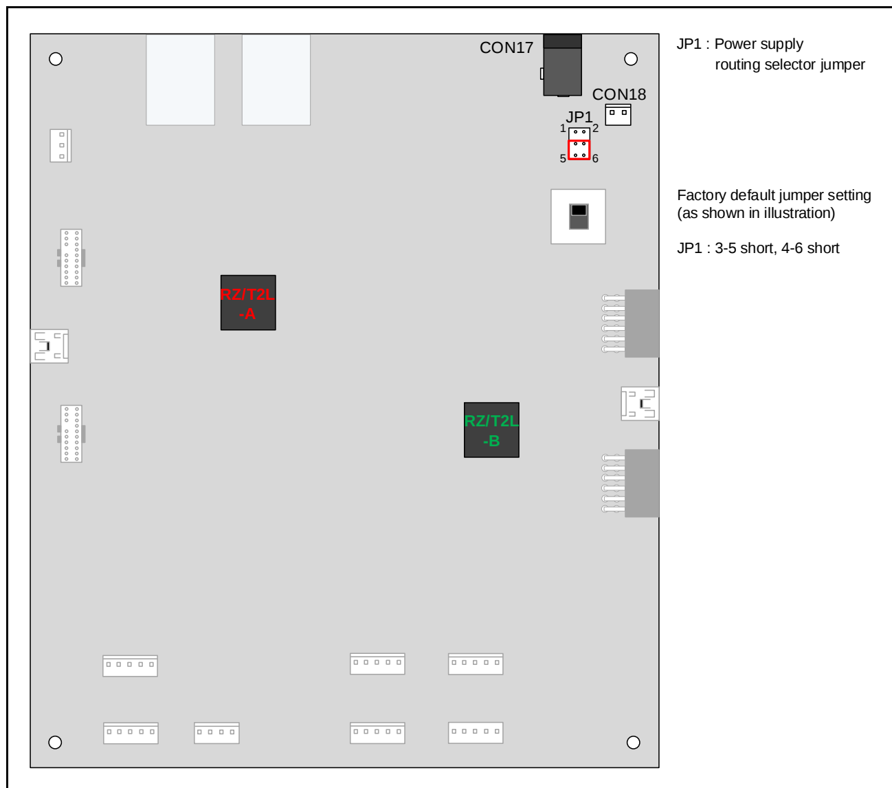
Figure 4.3.1 Functional Safety Reference Board - Jumper Position (C side Up)
