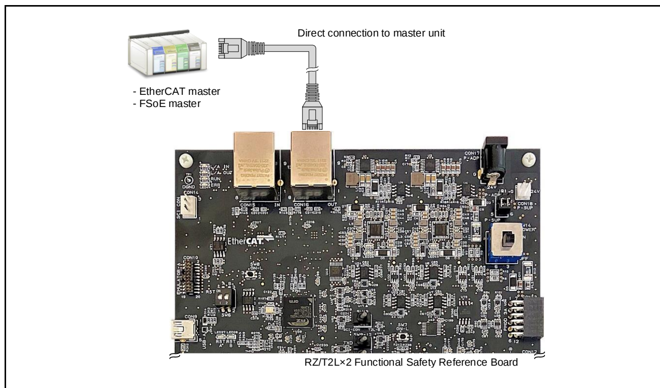
Figure 2.3.2 System Configuration Example for FSoE Reference Purpose
