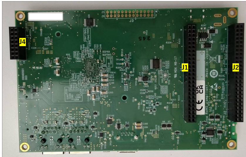
Figure 3.1-2 RZ/V2N Evaluation Board Layout Diagram (Solder Side)
