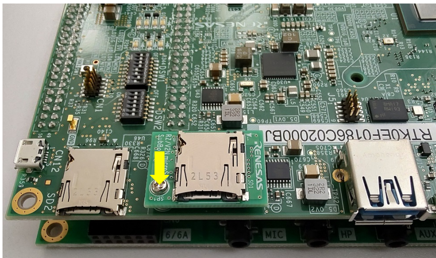
Figure 2.1-4 Use Screw to Fix Sub Board (the photo shows an installed microSD Sub Board)
