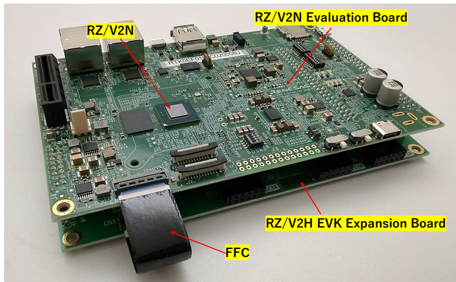
Figure 1.3-1 Outer Appearance of V2NEVK
