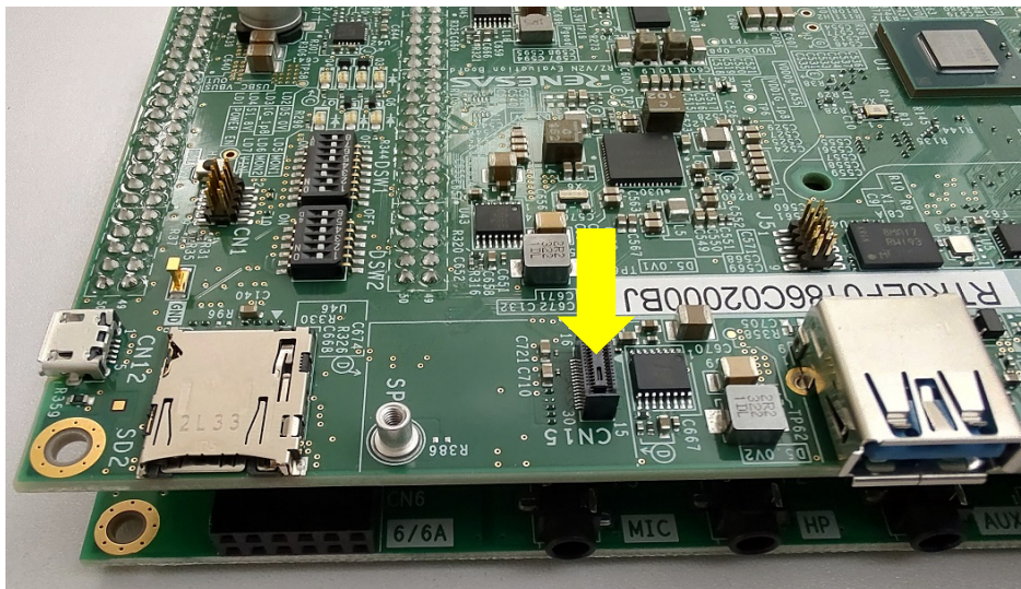
Figure 2.1-3 Connect Sub Board to RZ/V2N Evaluation Board
