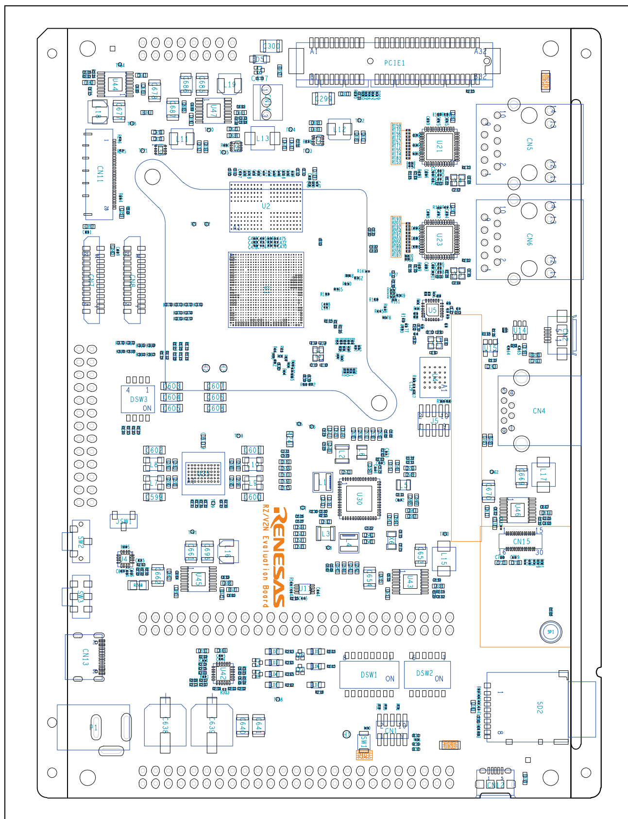
Appendix A.1 Parts Layout (Top)
