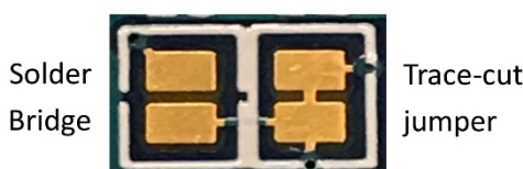
Figure 4. Copper Jumpers
