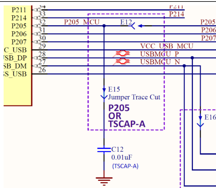
Figure 32. P205 Circuit
