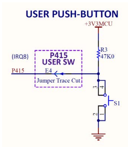
Figure 16. User Switch Circuit
