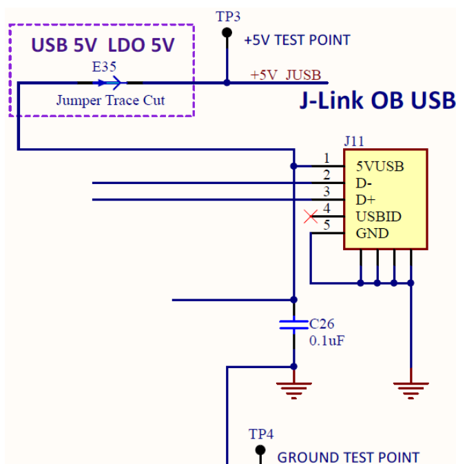
Figure 9. 5 V Power Input Circuit
