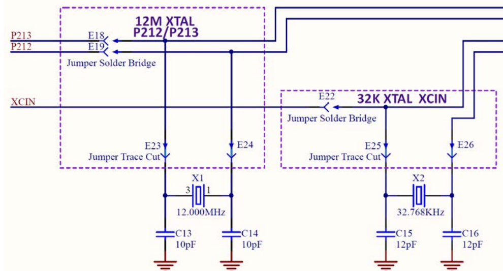
Figure 26. Crystal Clock Sources
