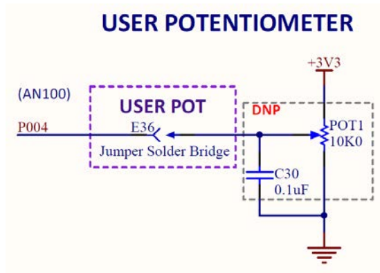
Figure 27. User Potentiometer Circuit
