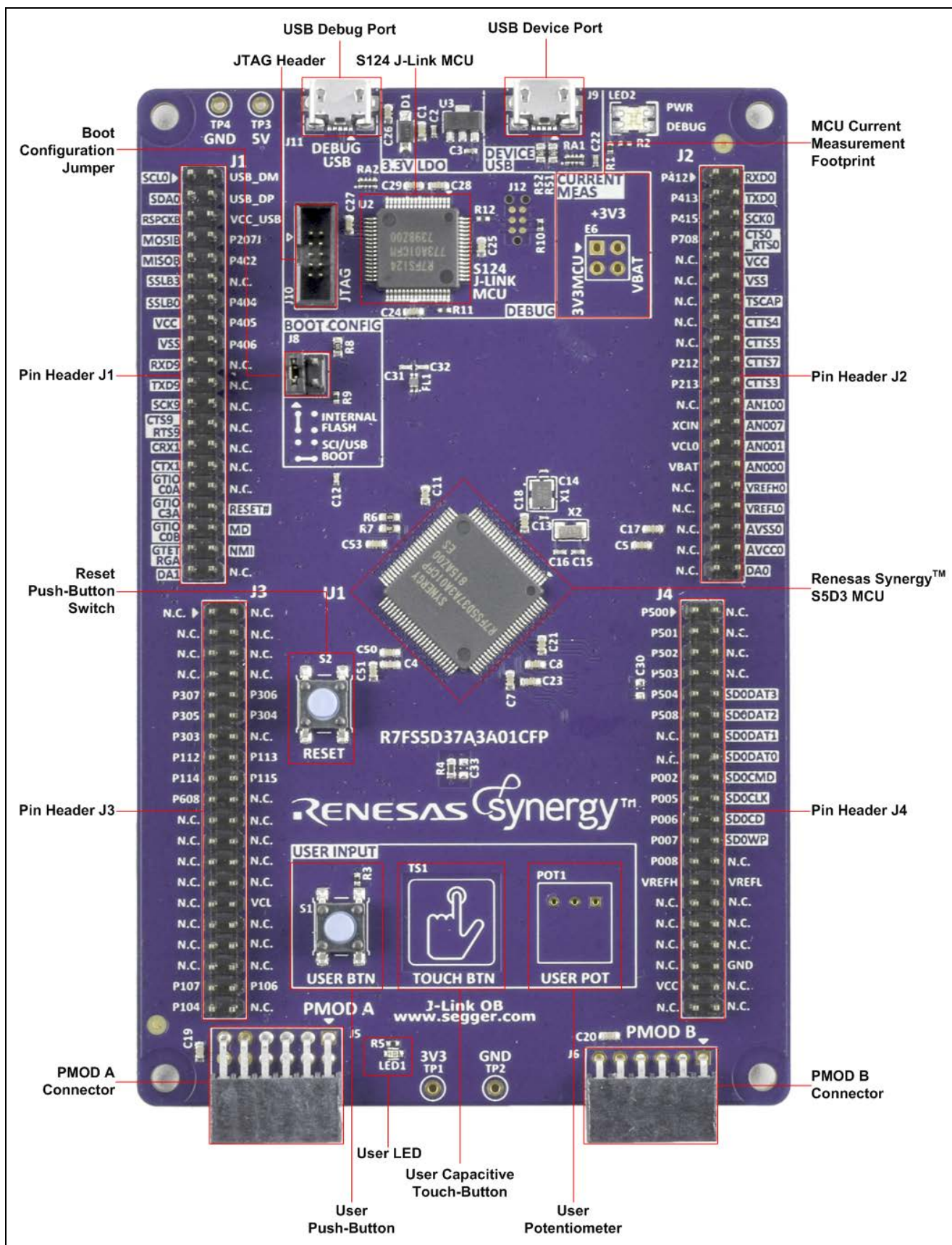
Figure 1. TB-S5D3 Top Side
