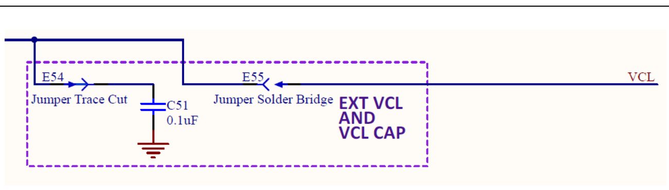
Figure 30. VCL and VCL Capacitor
