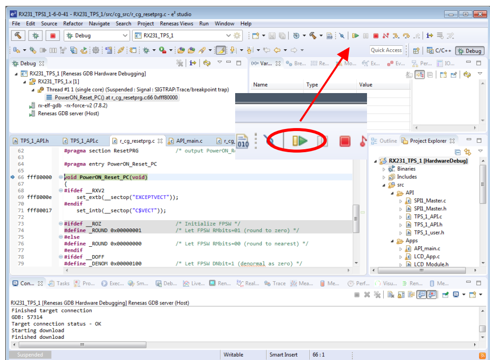
Figure 3-7: Debug perspective
