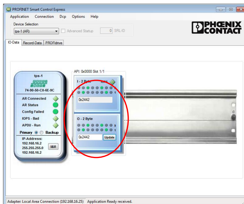
Figure 4-11 PROFINET Smart Control operation
