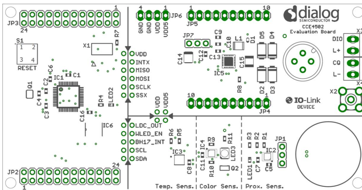
Figure 10: Layout Assembly
