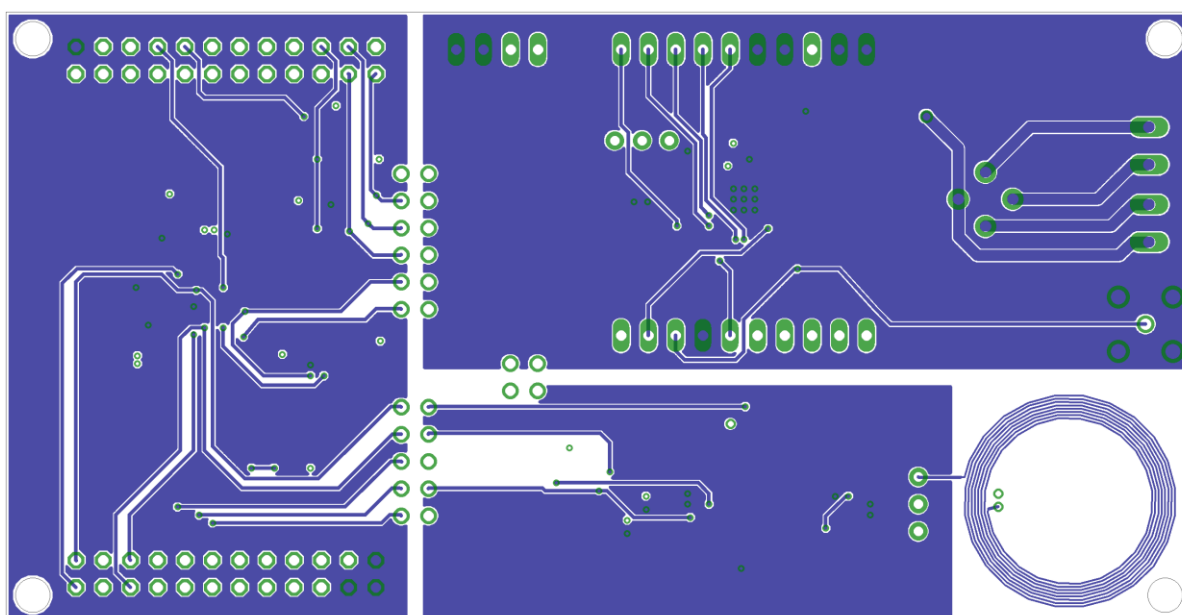
Figure 9: Layout BOTTOM
