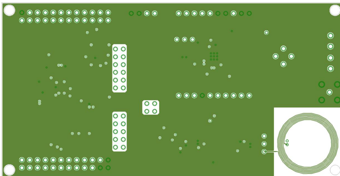
Figure 8: Layout MID 2
