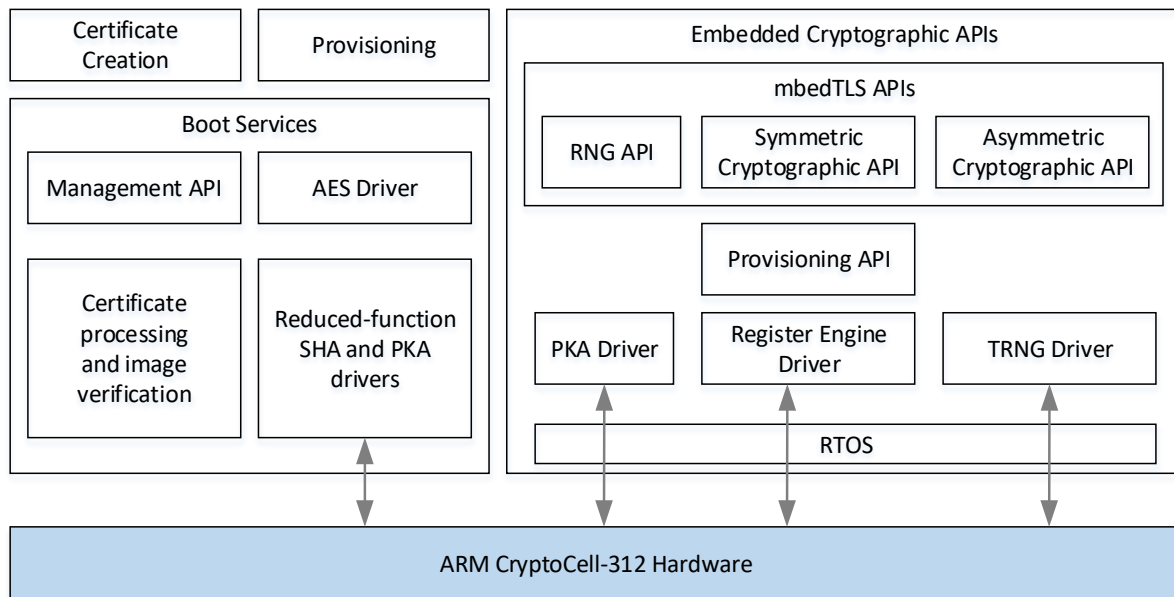
Figure 2. DA16200/DA16600 security software architecture
