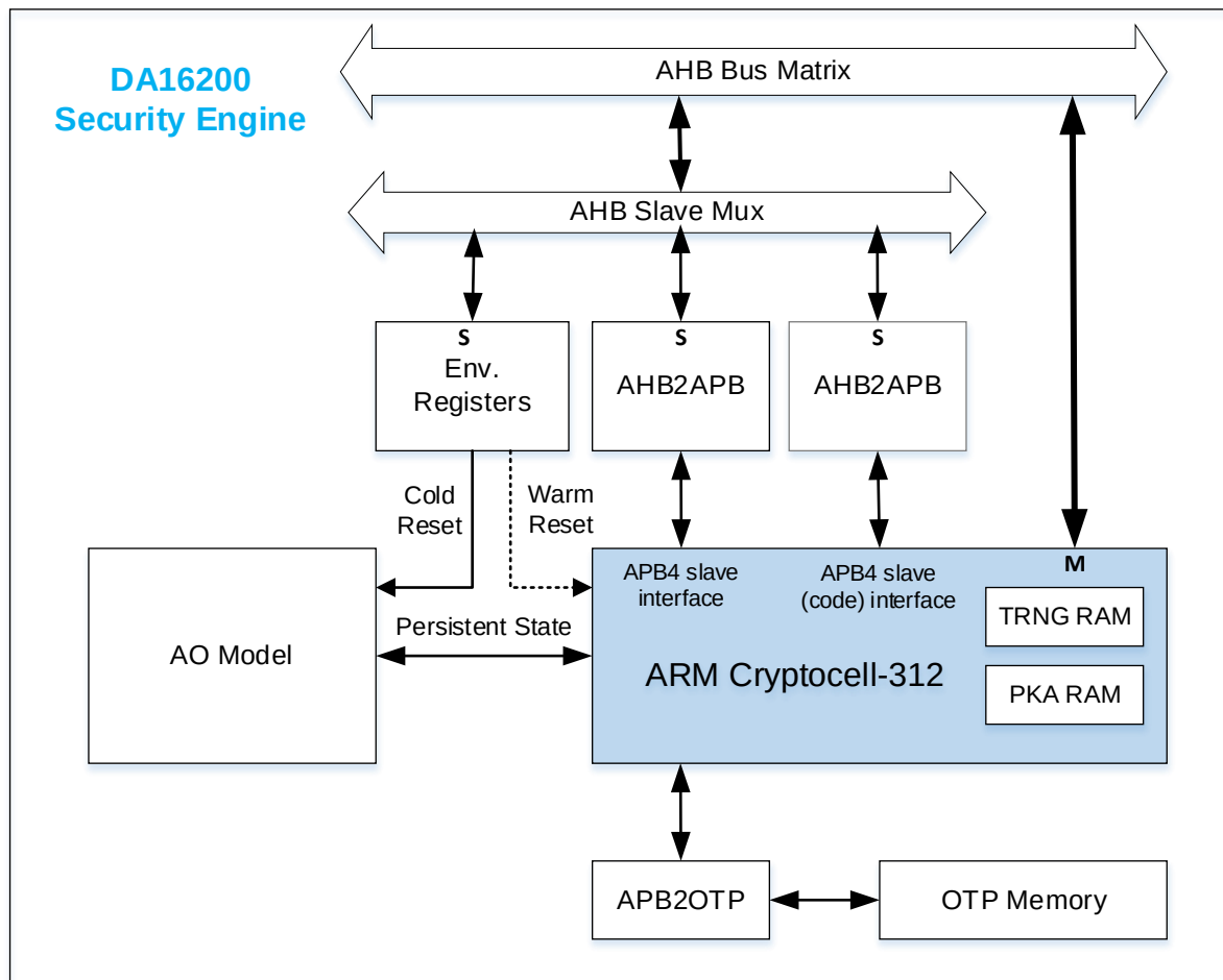
Figure 1. Block diagram of DA16200/DA16600 security engine
