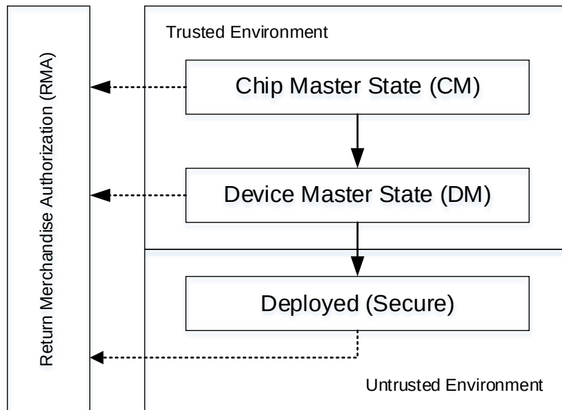
Figure 3. LCS transitions
