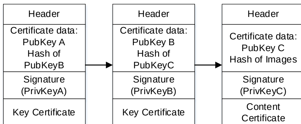
Figure 5. Three-certificate chain
