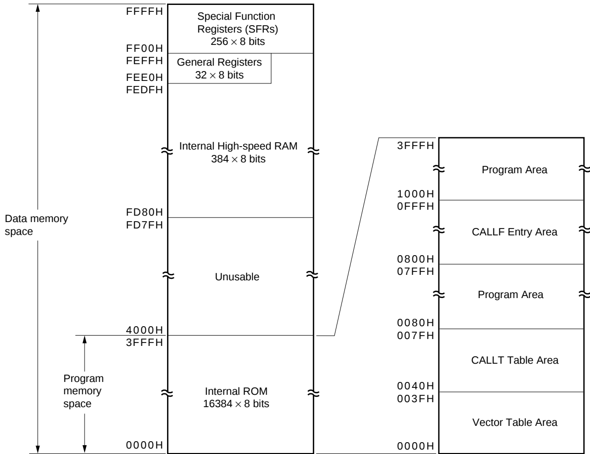
Figure 3-2. Memory Map ( \mu PD78082)
