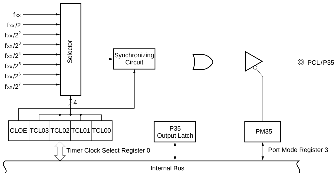
Figure 8-2. Clock Output Control Circuit Block Diagram
