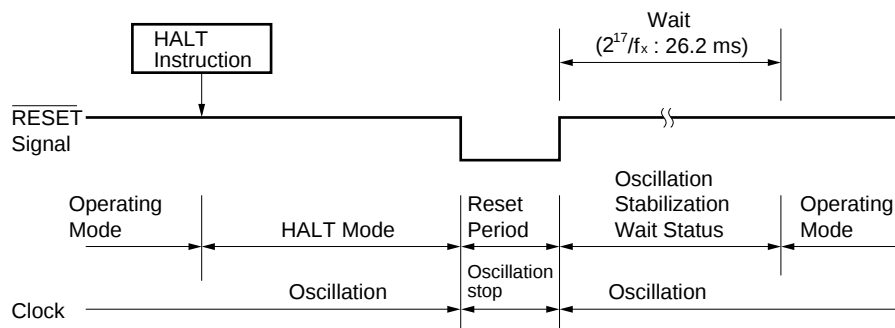
Figure 13-3. HALT Mode Release by RESET Input
