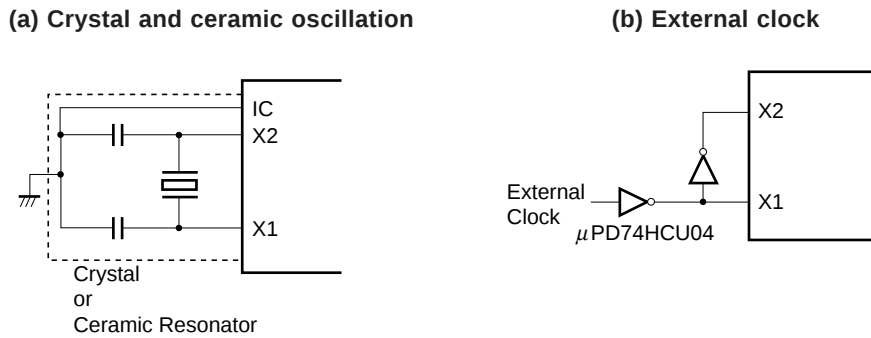
Figure 5-5. External Circuit of Main System Clock Oscillator
