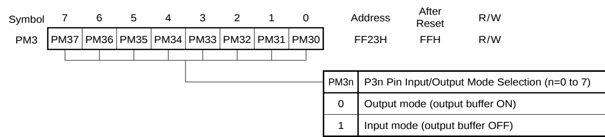
Figure 8-4. Port Mode Register 3 Format
