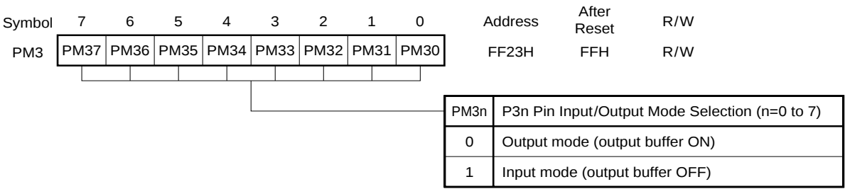
Figure 9-3. Port Mode Register 3 Format
