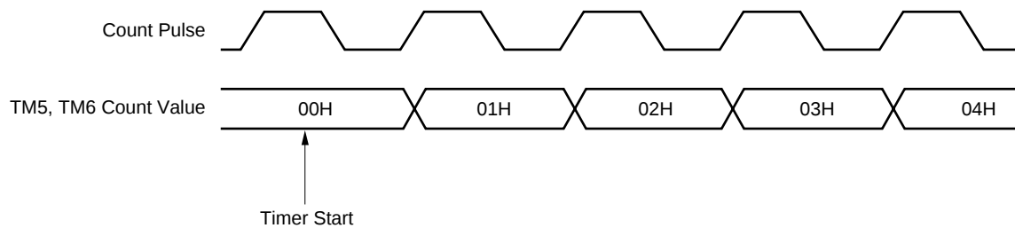
Figure 6-18. 8-Bit Timer Registers 5 and 6 Start Timing
