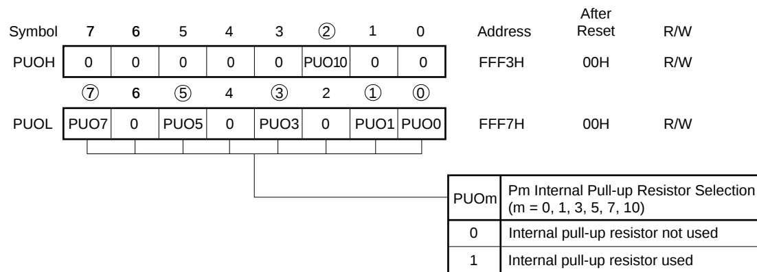
Figure 4-11. Pull-Up Resistor Option Register Format
