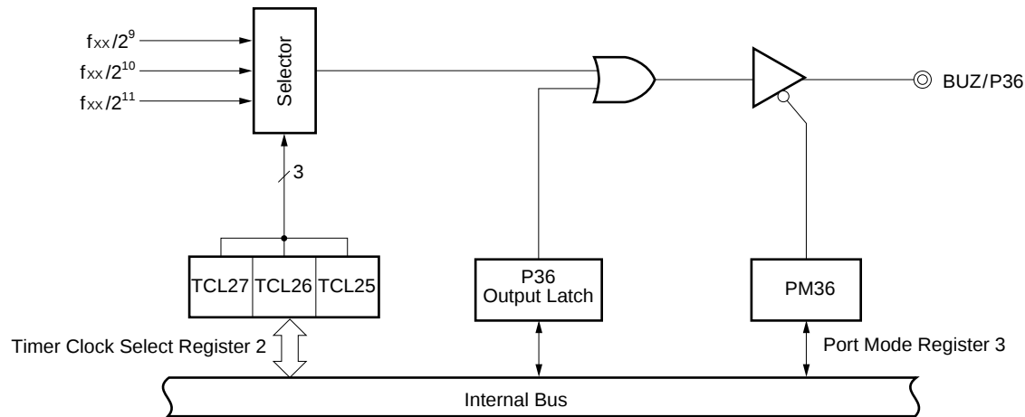
Figure 9-1. Buzzer Output Control Circuit Block Diagram
