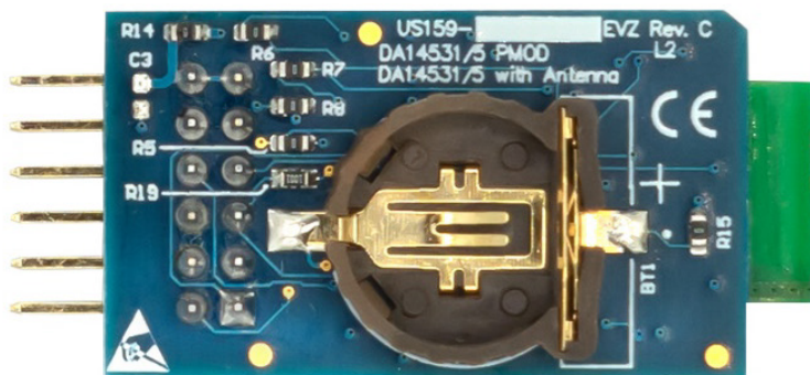
Figure 5. DA14535 EVB (Bottom)
