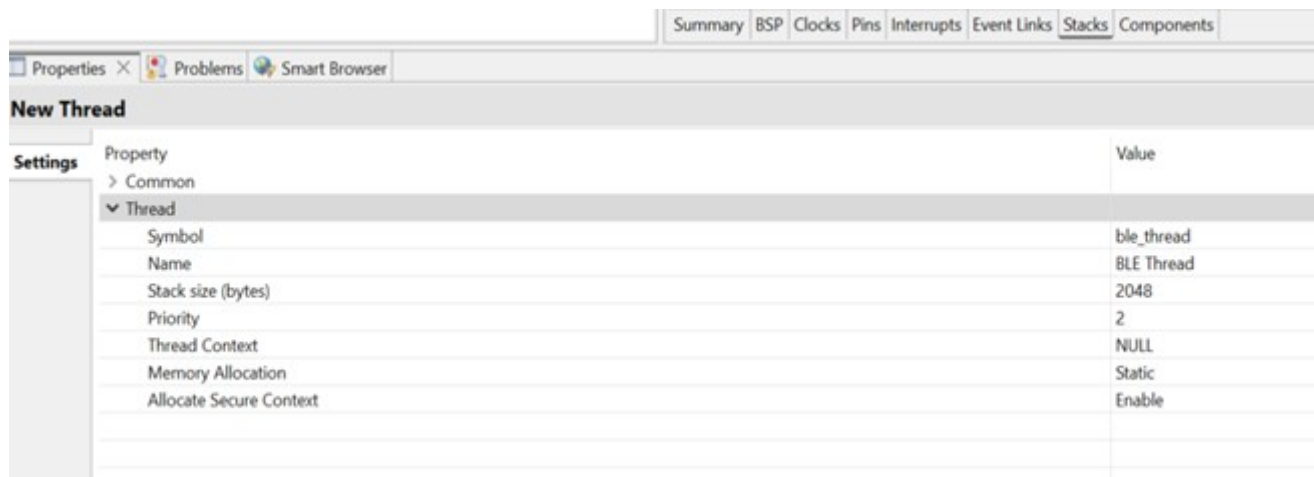
Figure 8. BLE Thread Configuration
