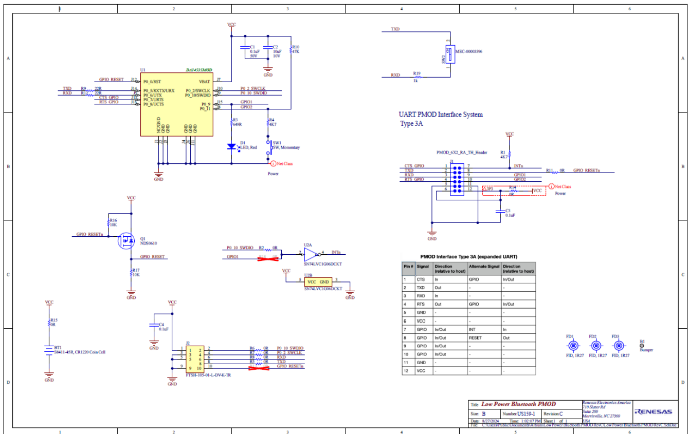
Figure 15. US159-DA14535EVZ Application Schematic Diagram
