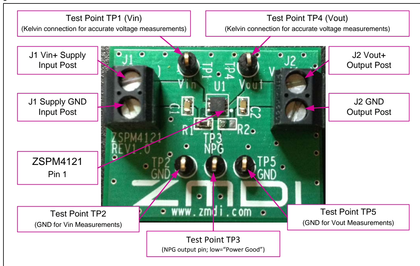
Figure 2.1 ZSPM4121 Evaluation Board Connections
