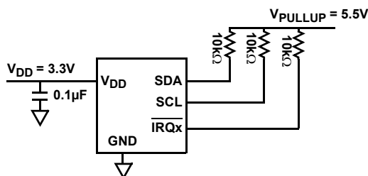
FIGURE 1. EXAMPLE CIRCUIT WITH V_{DD} AT 3.3V AND I 2 C AND IRQX PULLED UP TO 5.5V
