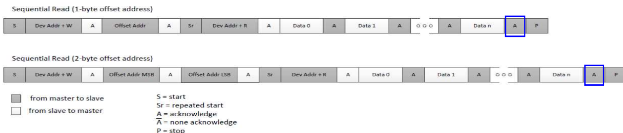
Figure 4. I 2 C Master Read Cycle Sequencing
