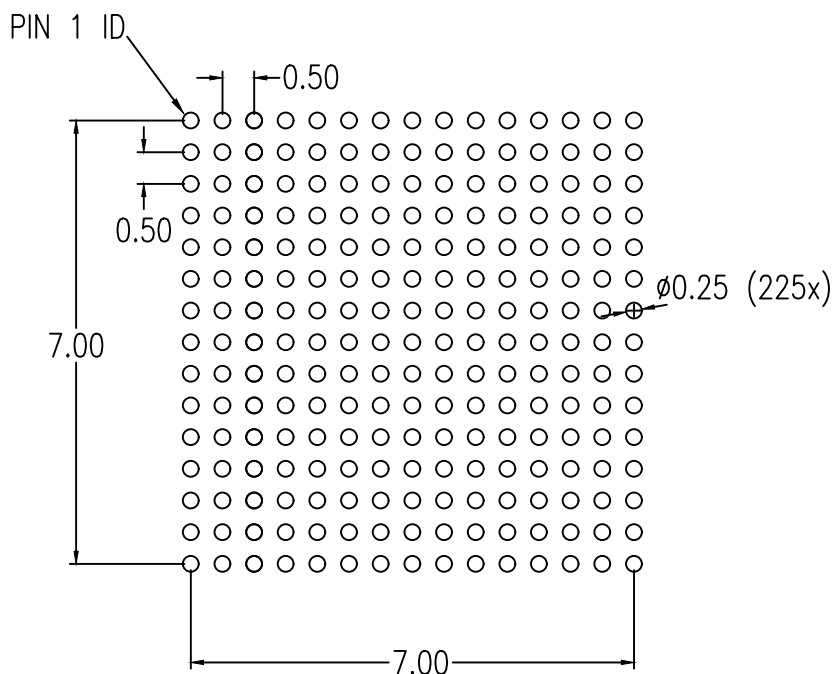
RECOMMENDED LAND PATTERN DIMENSION (TOP VIEW)
