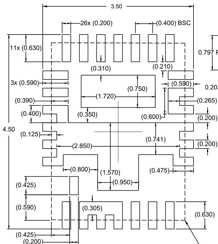
Recommended Land Pattern
