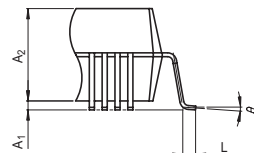
Detail F
