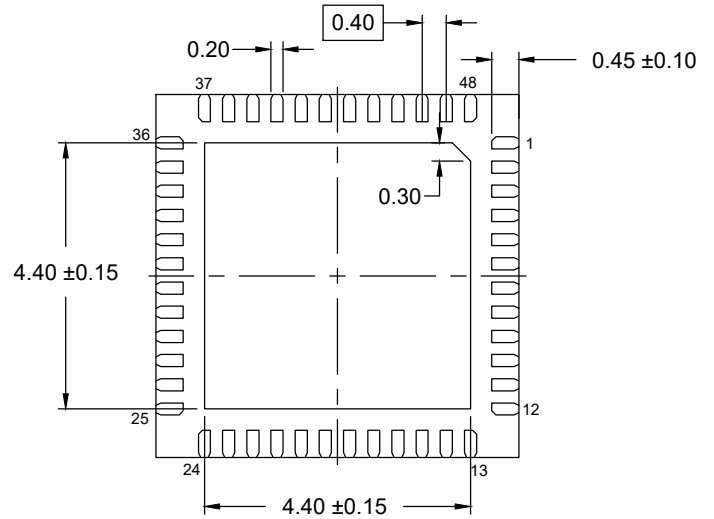
Bottom View
