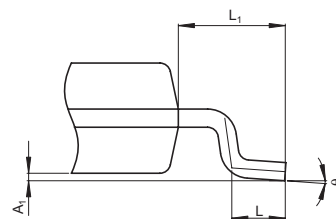
Detail F
