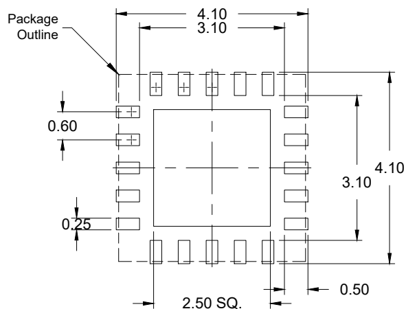
RECOMMENDED LAND PATTERN (PCB Top View)
