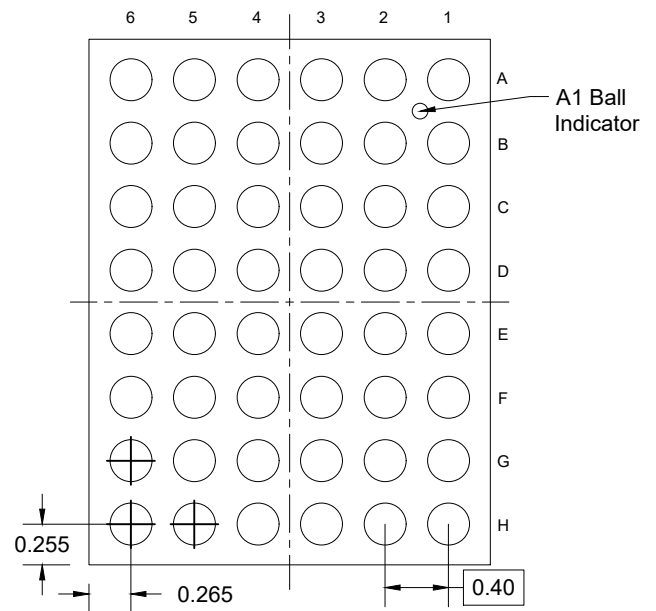
BOTTOM VIEW
