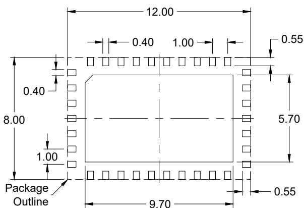
RECOMMENDED LAND PATTERN (PCB Top View)
