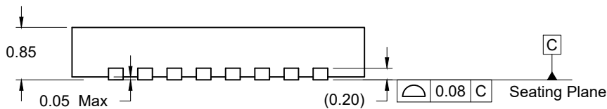
SIDE VIEW
