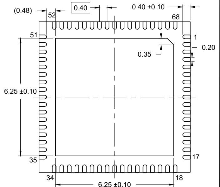
BOTTOM VIEW
