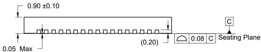
SIDE VIEW
