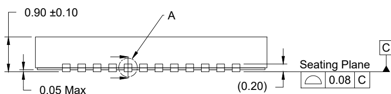
SIDE VIEW
