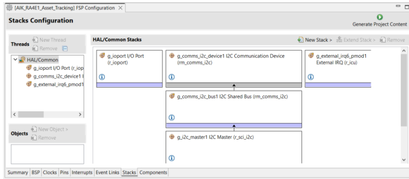
Figure 11. Opening the Configurator
