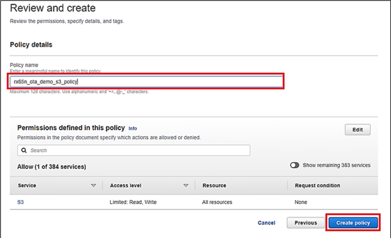
Figure 97. Create inline policy (3/3)
