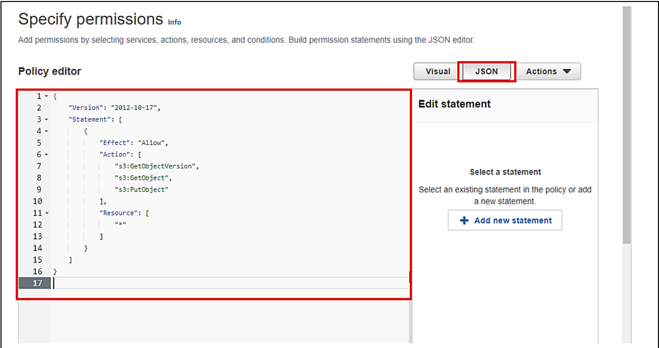
Figure 96. Create inline policy (2/3)
