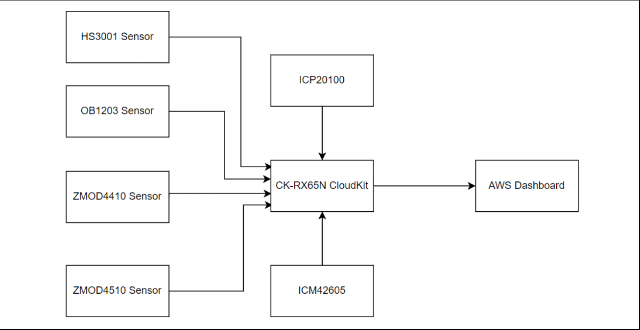
Figure 2. System Diagram
