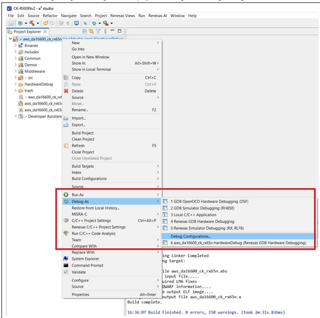
Figure 20. Configuration Debugger 1/2
