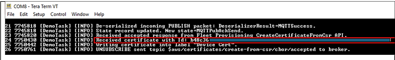
Figure 181. Running Application with Fleet (8/8)
