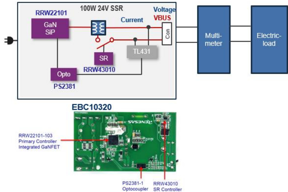
Figure 1. EBC10320 Evaluation Board
