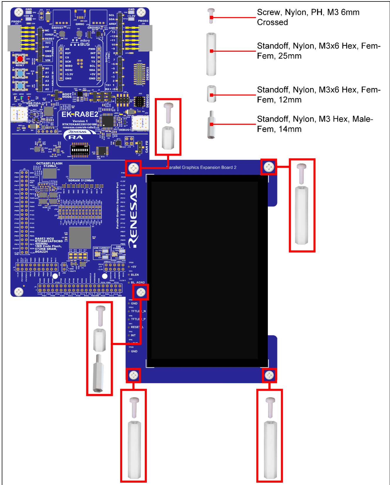
Figure 2. Parallel Graphics Expansion Board 2 connected to the EK-RA8E2
