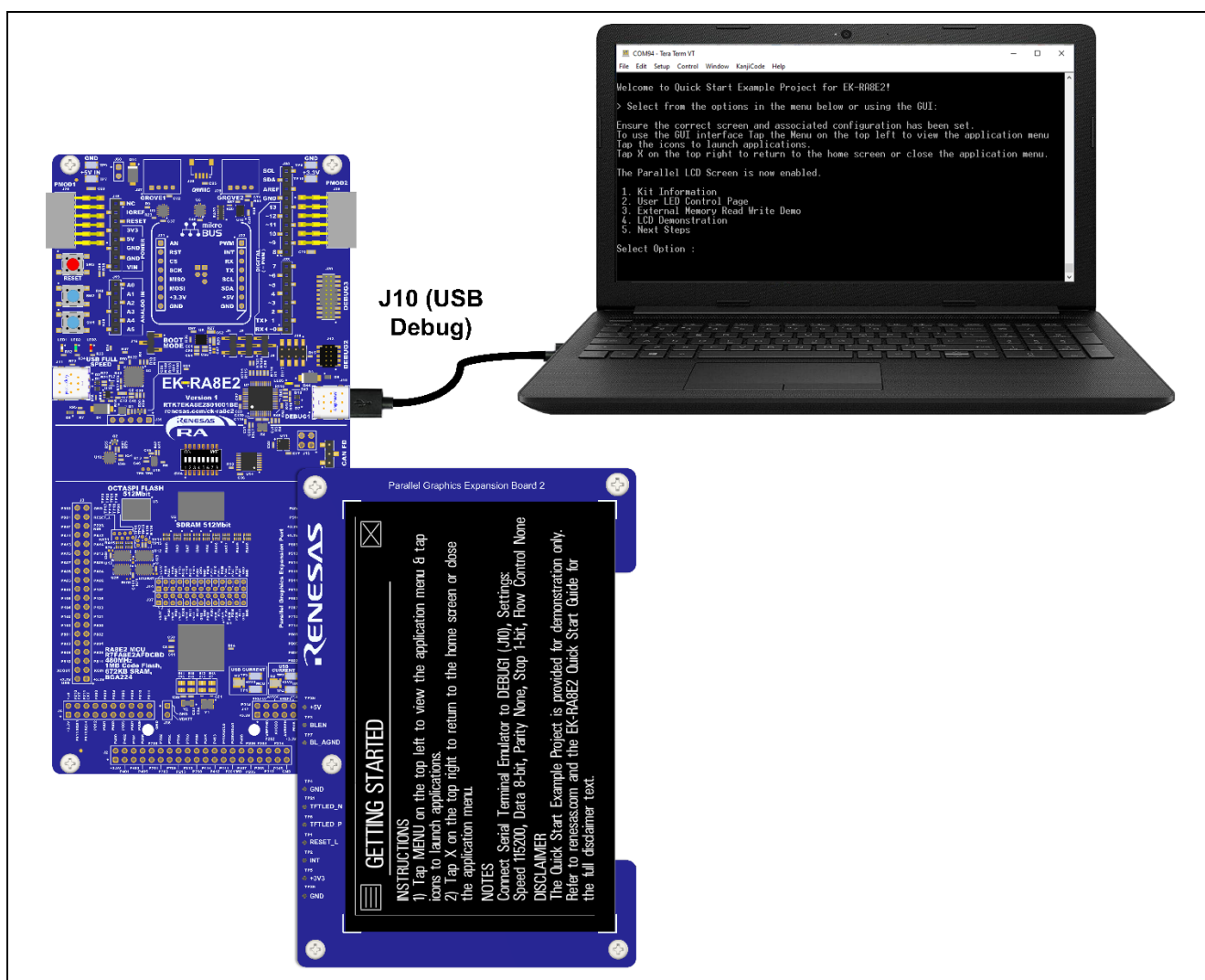
Figure 4. Connecting the EK-RA8E2 Board to the Host PC via USB Debug
