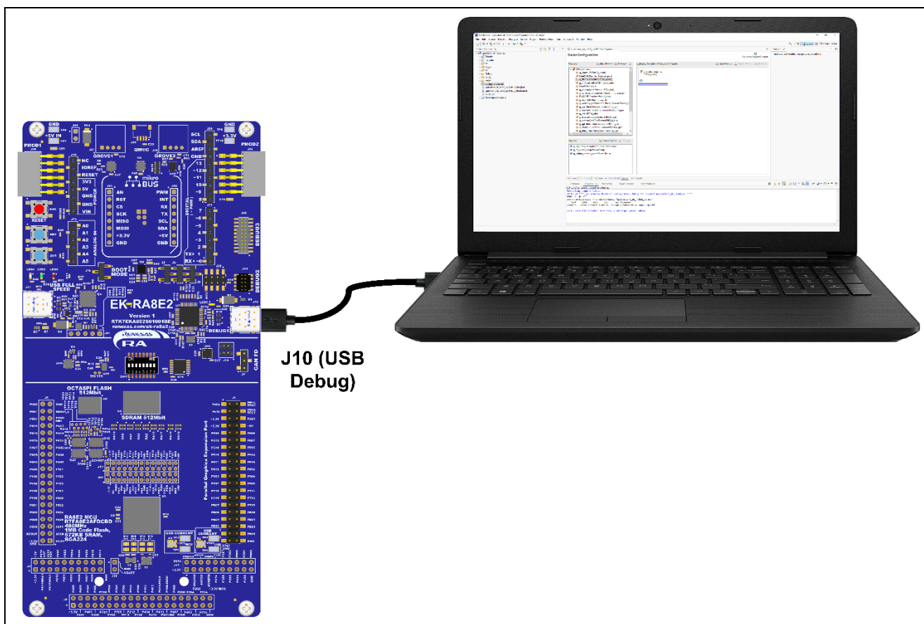
Figure 37. Connecting the EK-RA8E2 Board to the Host PC via USB Debug Port
