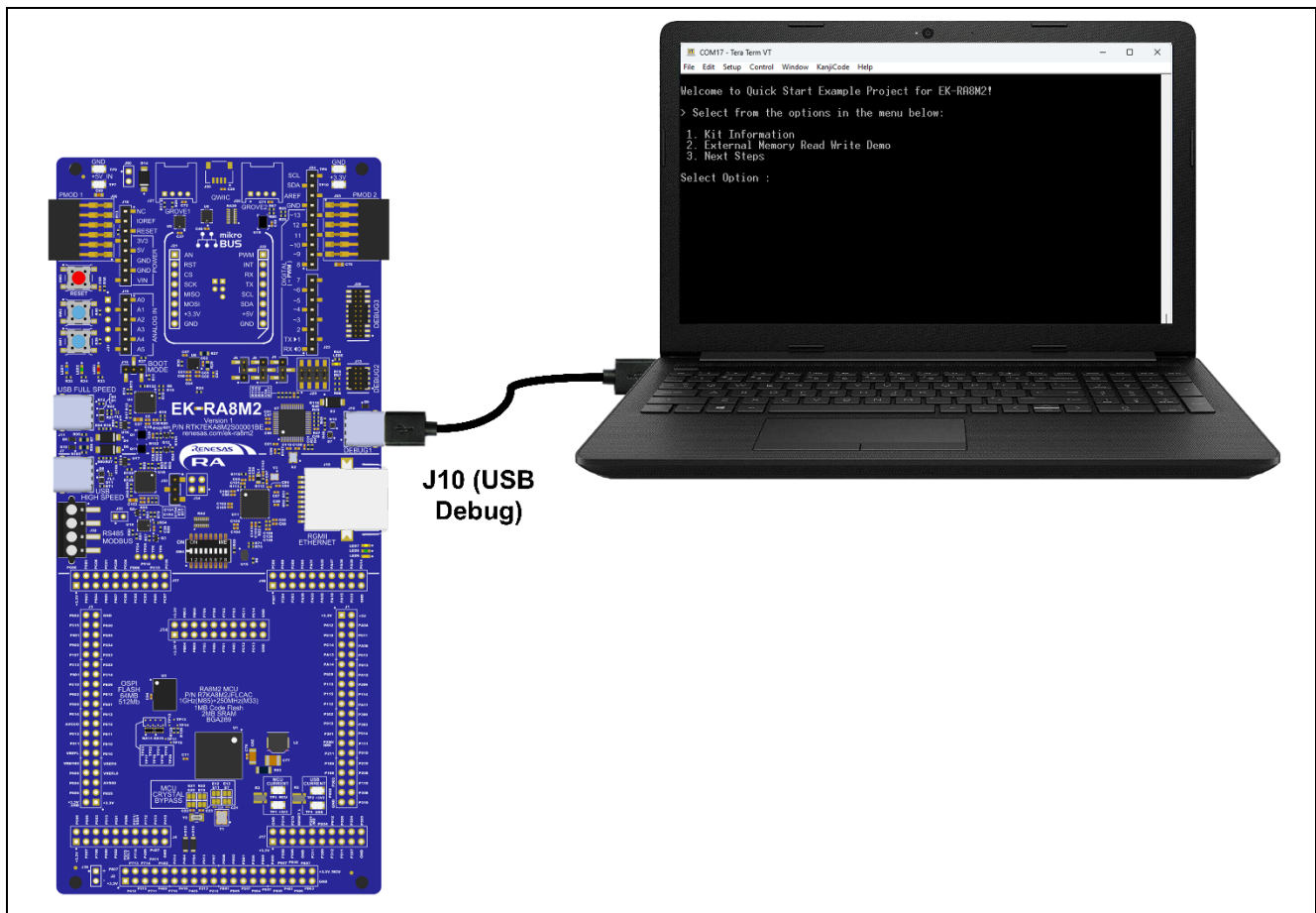
Figure 3. Connecting the EK-RA8M2 Board to the Host PC via USB Debug
