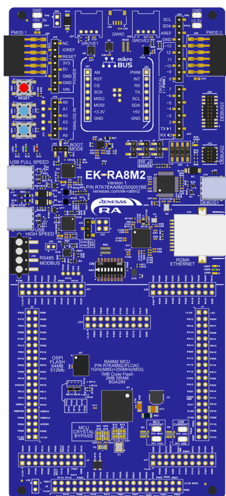
Figure 1. EK-RA8M2 Kit Contents
