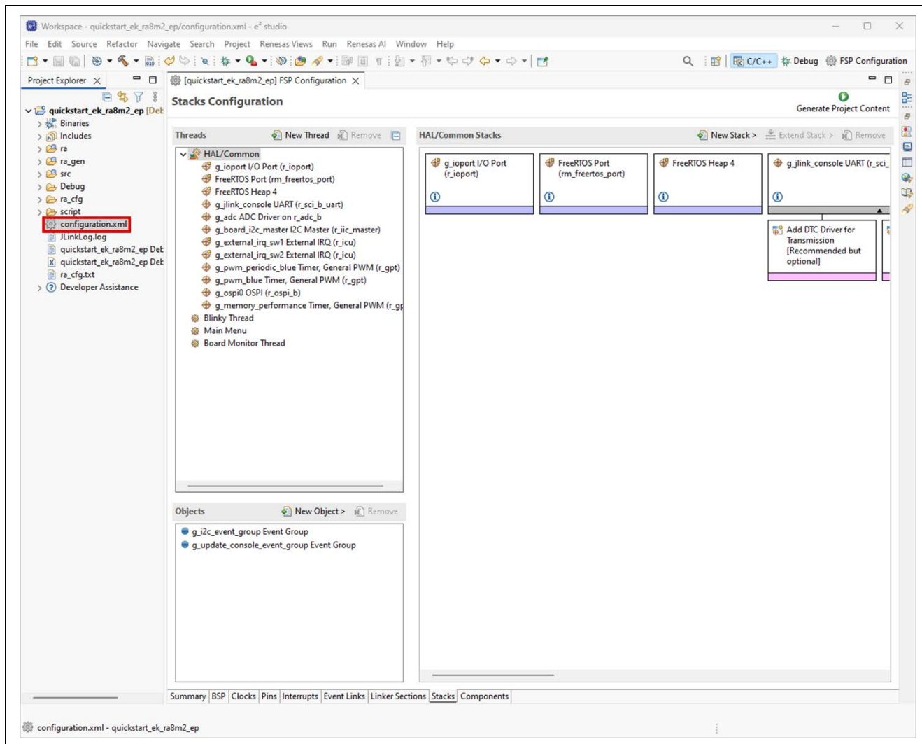
Figure 19. Opening the Configurator
