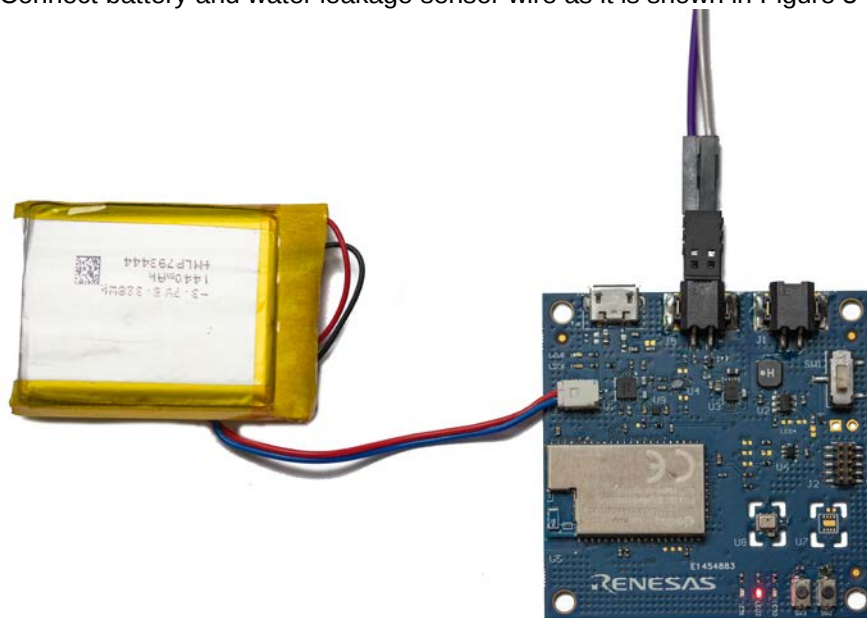
Figure 3. Battery and Water Leakage Sensor connection
