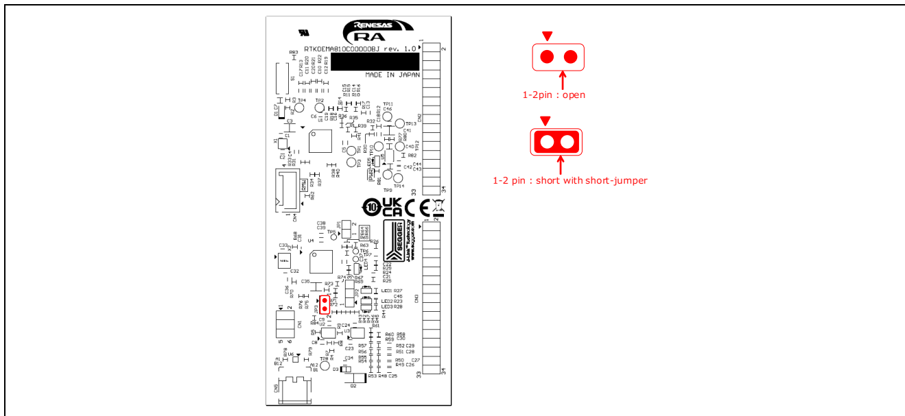
Figure 4-2 Jumper pin setting of CPU Board
