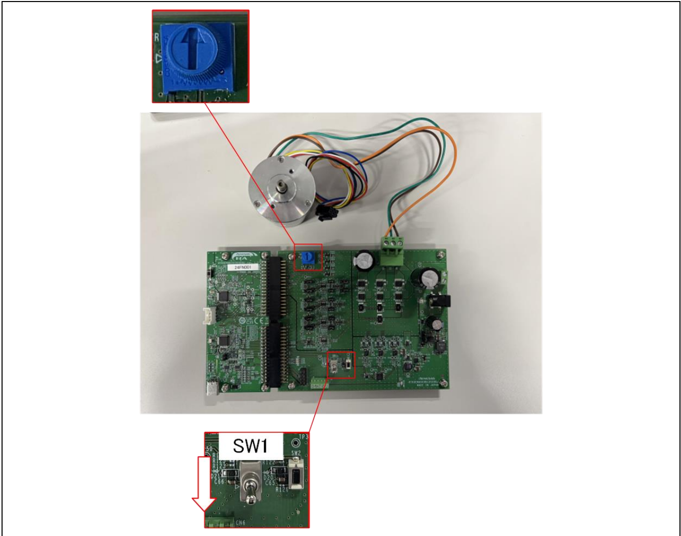
Figure 4-4 Hardware configuration
