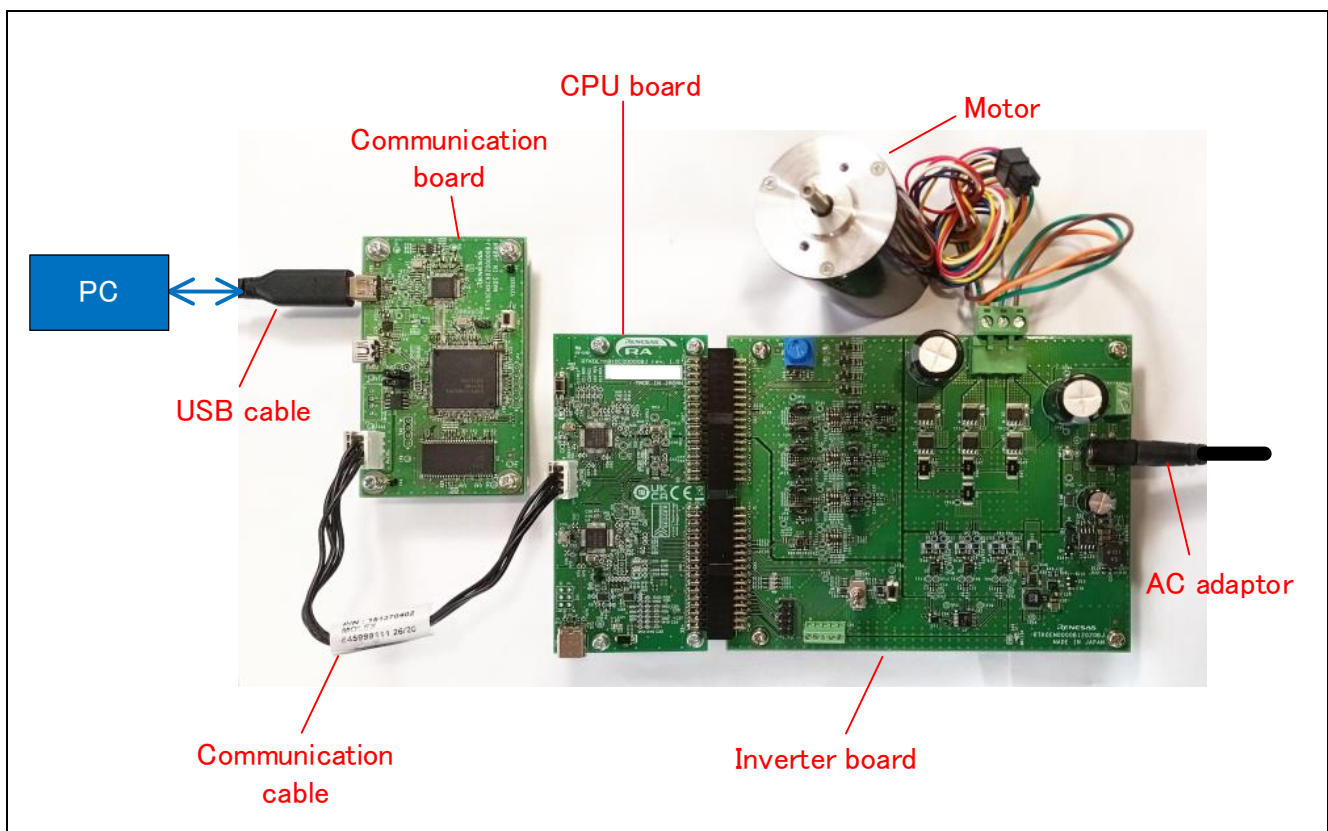
Figure 6-1 Hardware Configuration
