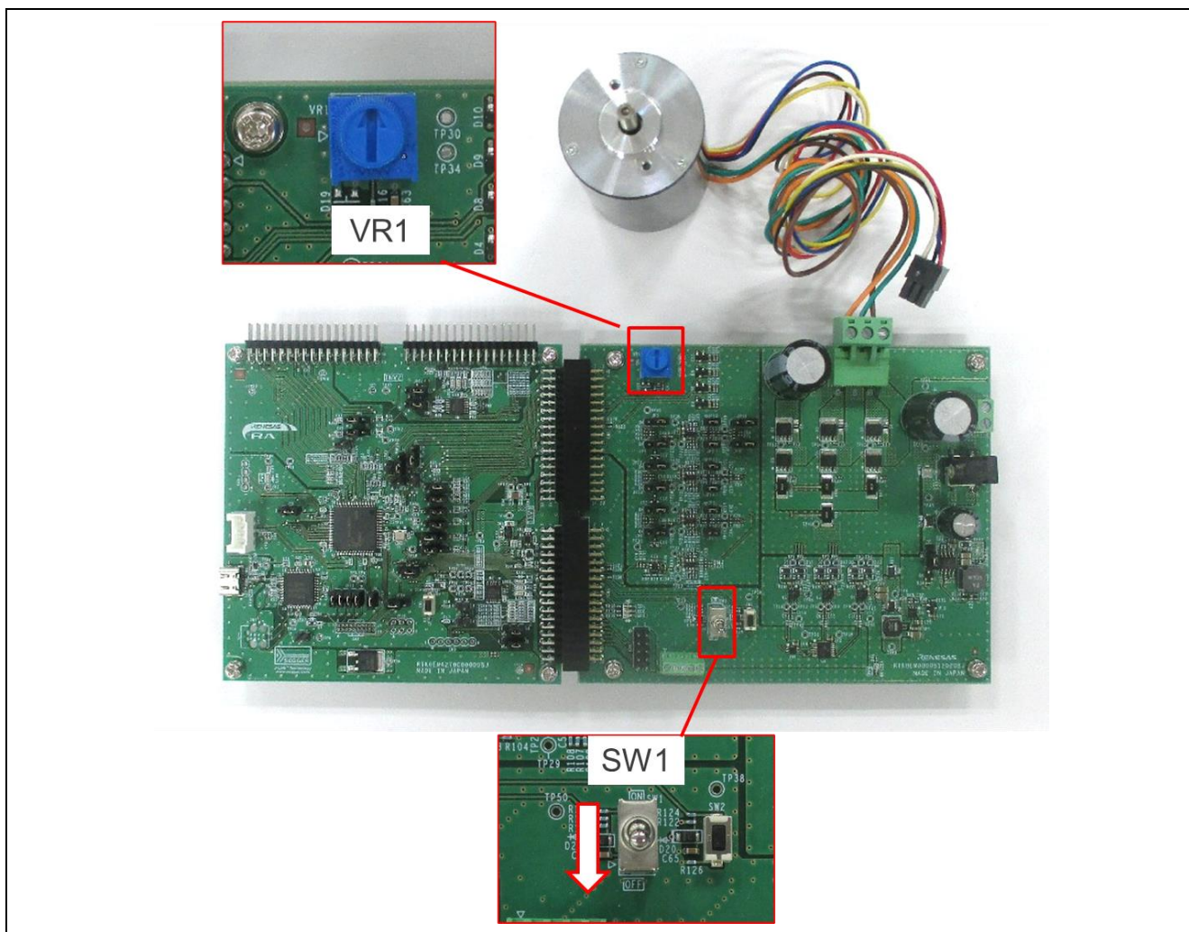
Figure 4-4 Hardware configuration
