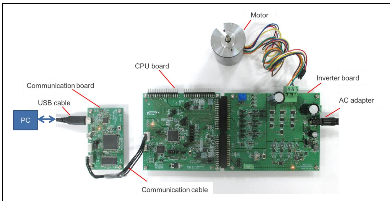
Figure 6-1 Hardware Configuration
