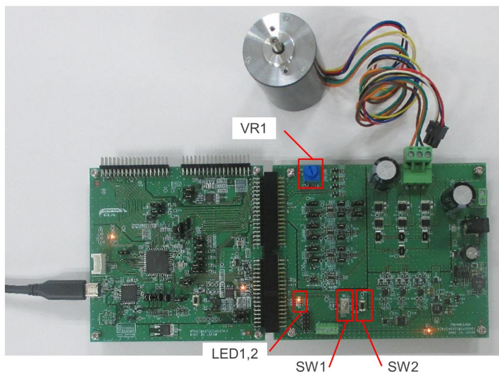
Figure 4-6 Operating State
