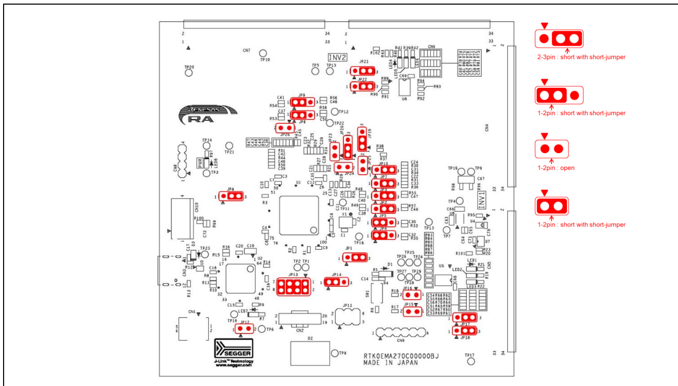
Figure 4-2 Jumper pin setting of CPU Board
