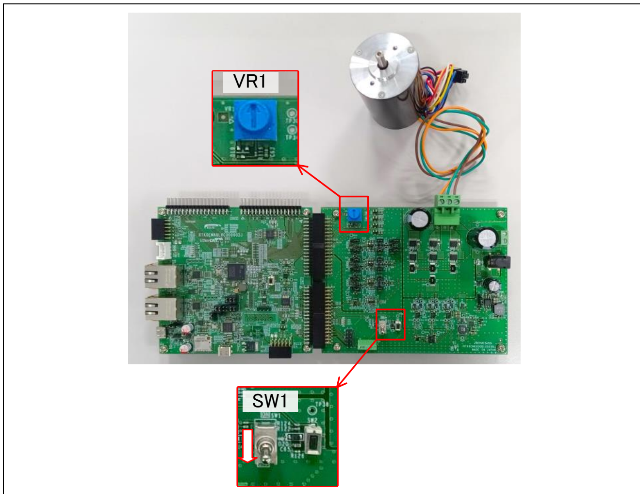
Figure 4-4 Hardware configuration
