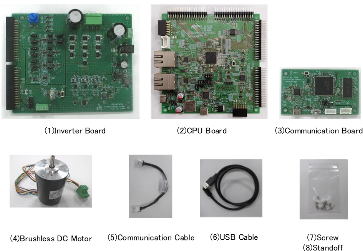
Figure 2-1 Product contents
