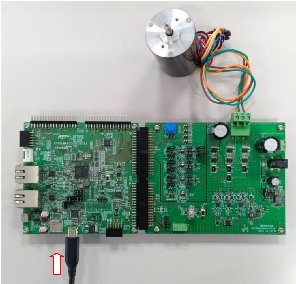
Figure 4-5 Power Supply
