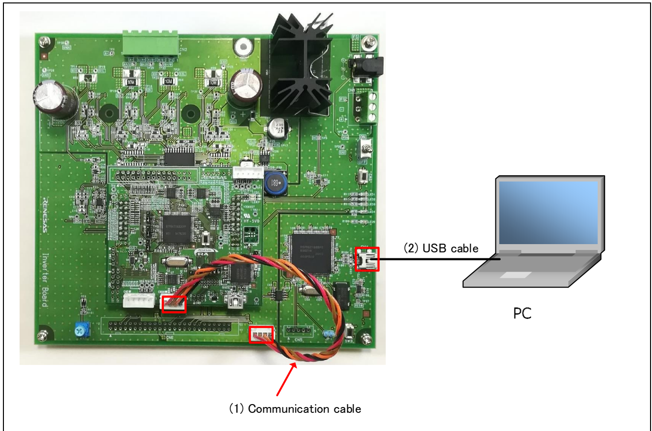
Figure 5-1 Connect cables
