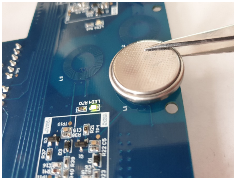
Figure 9. Conductive target detection illuminating LED
