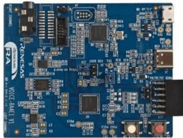
Figure 1. VOICE-RA4E1 Kit
