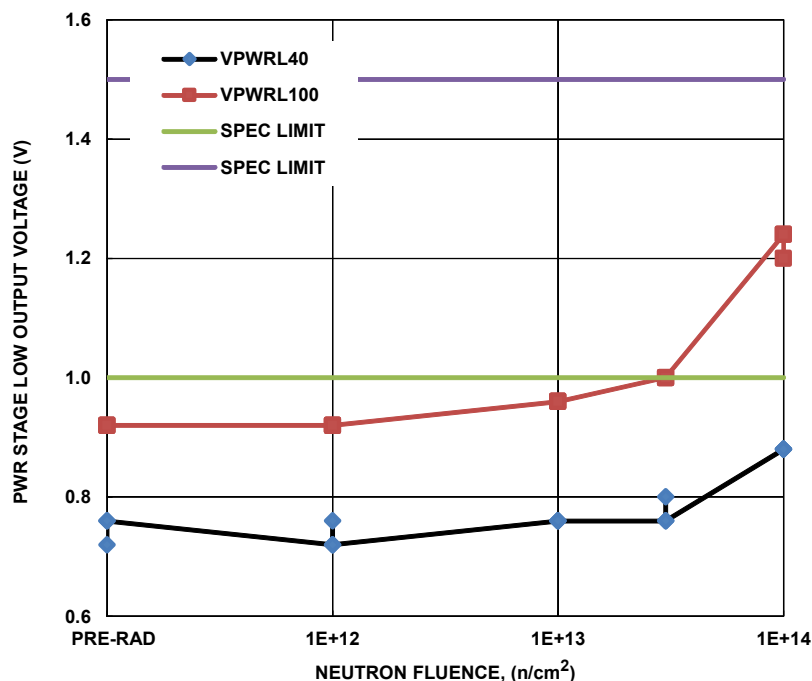
FIGURE 7. IS-1715ARH PWR stage saturated LOW output voltage, 40mA and 100mA load current cases, as a function of neutron irradiation, showing the median, minimum, and maximum of the populations following irradiation to each level. Neutron fluences and sample sizes (in parentheses) were 1 \times 10^{12} \text{ n/cm}^2 (five samples), 1 \times 10^{13} \text{ n/cm}^2 (five samples), 3 \times 10^{13} \text{ n/cm}^2 (five samples), and 1 \times 10^{14} \text{ n/cm}^2 (five samples). For reference, the post total dose SMD limits are 1V maximum (40mA load current case) and 1.5V maximum (100mA load current case).
