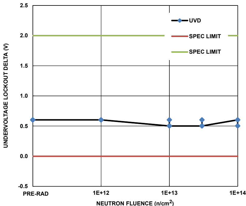
FIGURE 5. IS-1715ARH Undervoltage Lockout (UVLO) delta as a function of neutron irradiation, showing the median, minimum, and maximum of the populations following irradiation to each level. Neutron fluences and sample sizes (in parentheses) were 1 \times 10^{12} \text{ n/cm}^2 (five samples), 1 \times 10^{13} \text{ n/cm}^2 (five samples), 3 \times 10^{13} \text{ n/cm}^2 (five samples), and 1 \times 10^{14} \text{ n/cm}^2 (five samples). For reference, the post total dose SMD limits are 0V to 2V.
