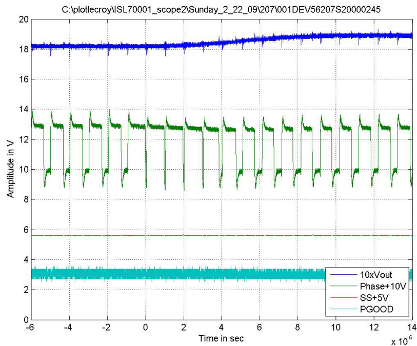
Figure 13. Non-Benign SET at LET = 43.2\text{MeV/mg/cm}^2
