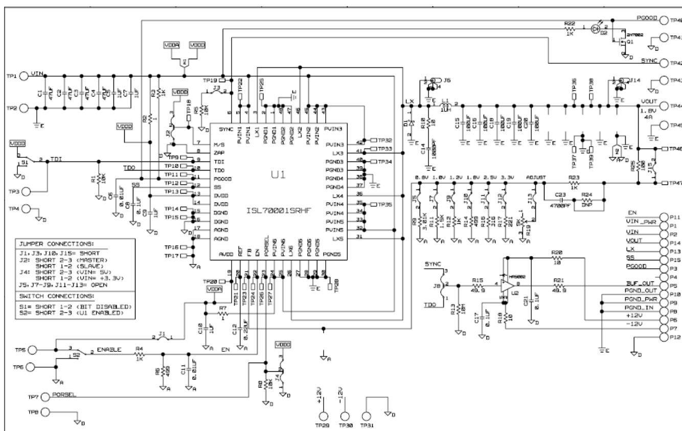
Figure 1. ISL70001SRH SEE Test Circuit Schematic
