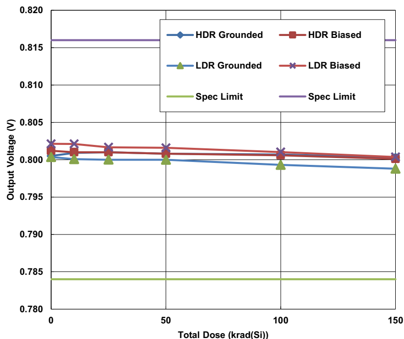
Figure 20. ISL70001SRH output voltage (3V supply) as a function of total dose irradiation at LDR and HDR for the unbiased (all pins grounded) and the biased (per Figure 2) cases. The LDR was 0.01rad(Si)/s and the HDR was 55rad(Si)/s. Sample size for each cell was 5. The SMD limits are \pm 2\% post-irradiation, which equals 0.784V to 0.816V for the 0.800V output voltage set point used for this test.
